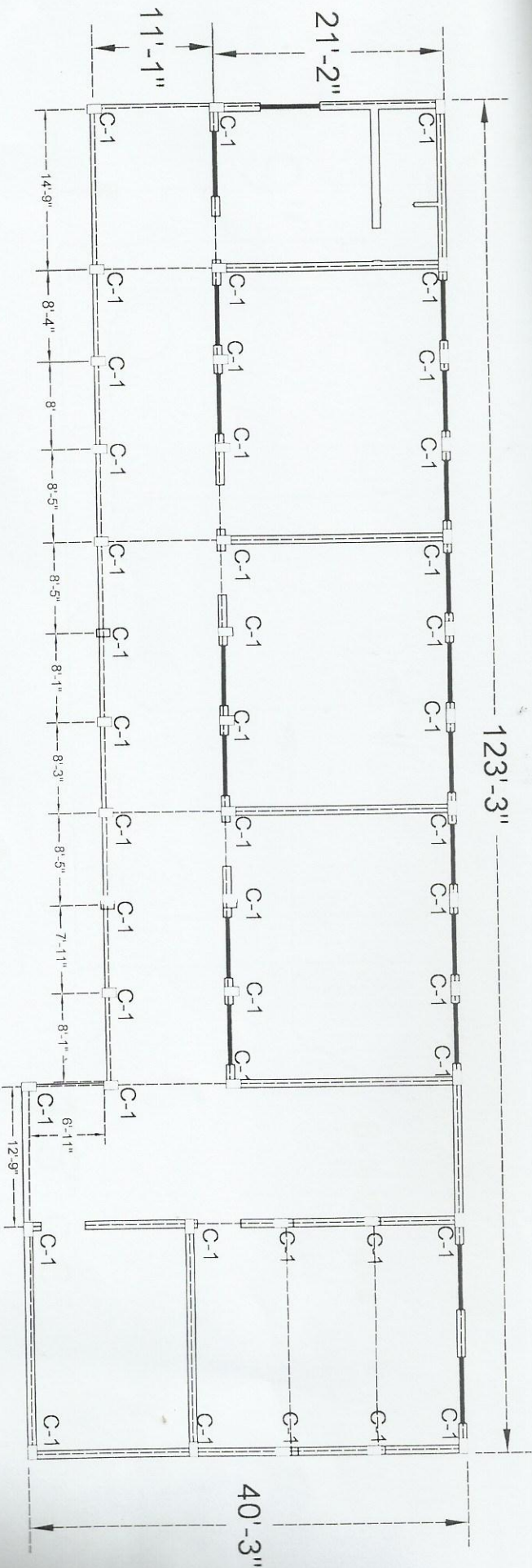
FIRST FLOOR DIMENSTION PLAN
