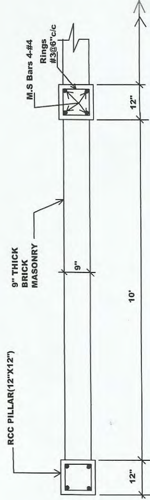
Plan
