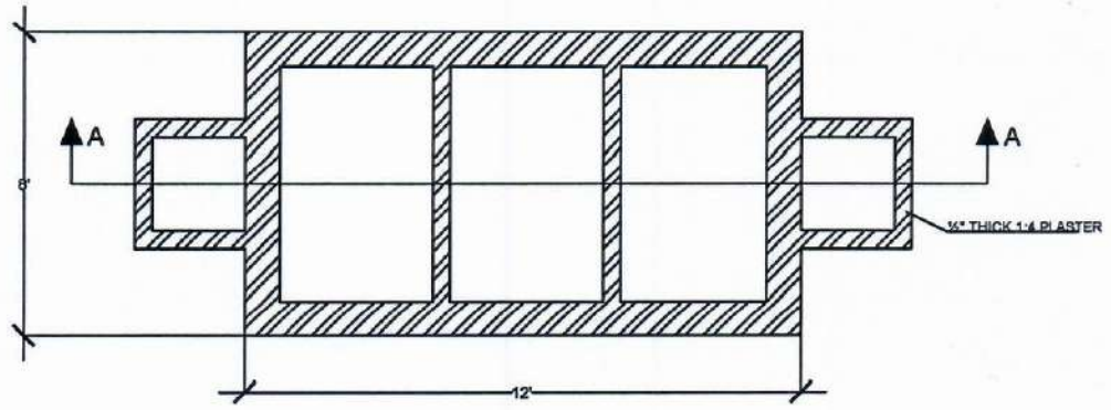
PROPOSED SEPTIC TANK 12'x8'x7'-6"
