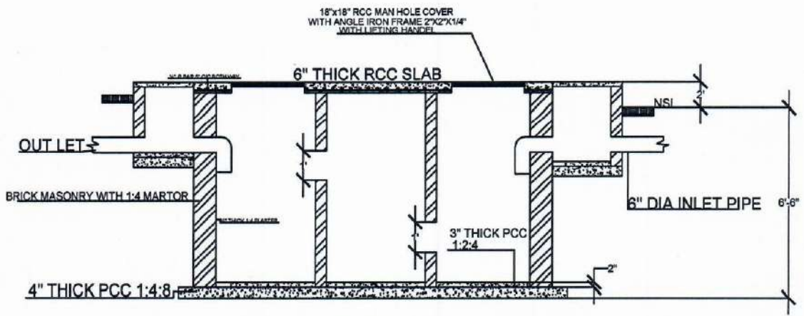
X-SEC AT A-A
