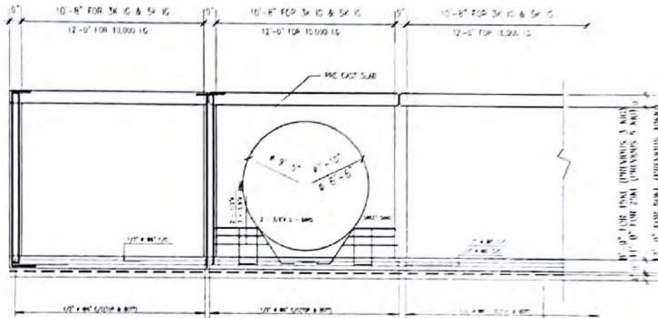
RCC PIT DETAIL
