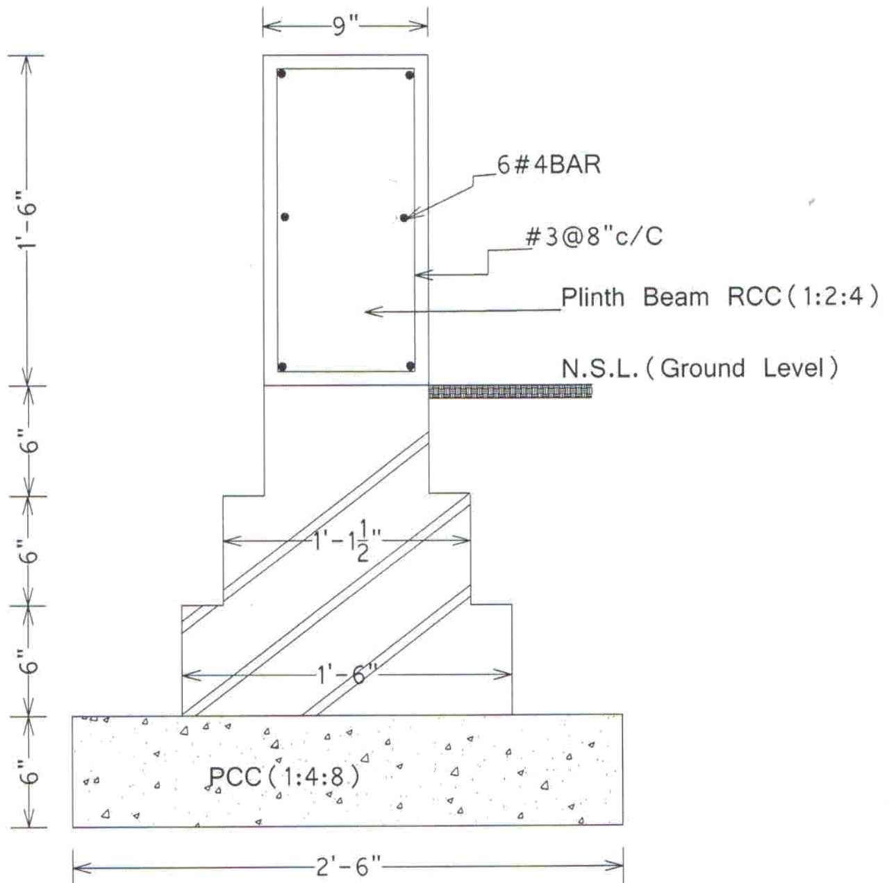
Foundation X-Section for Pre-Fab Structure
