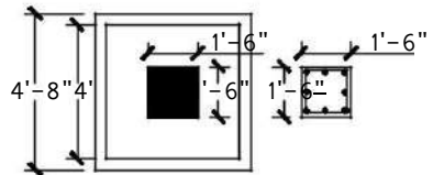
X-SECTION OF GATE COLUMN
