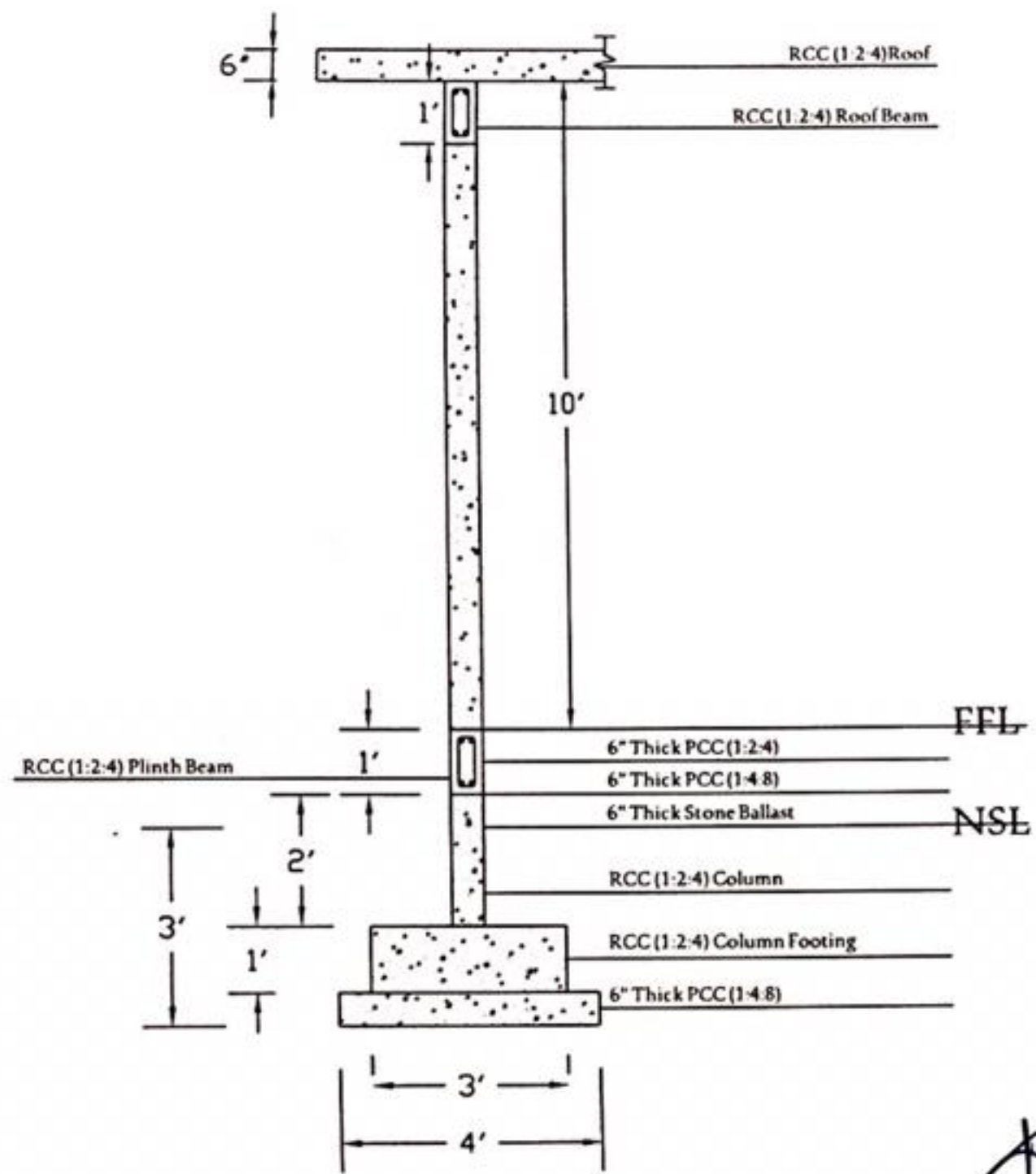
RCC Column Section
