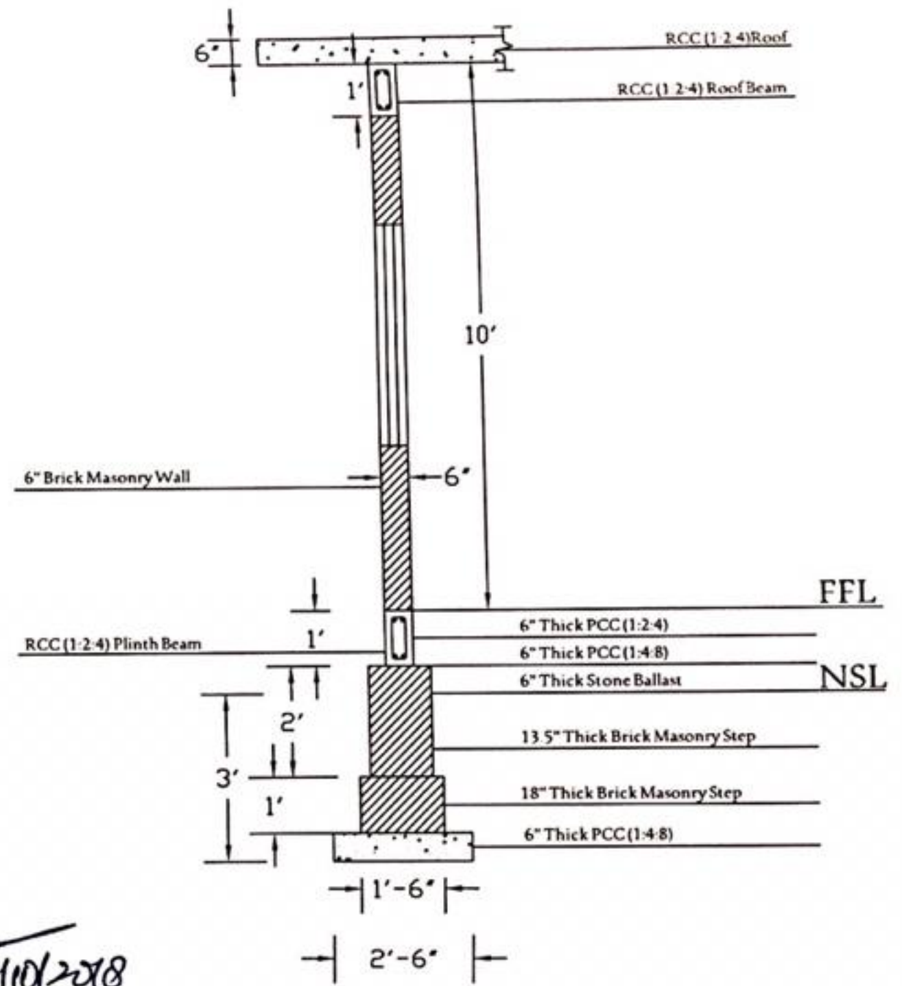
Brick Wall Section
