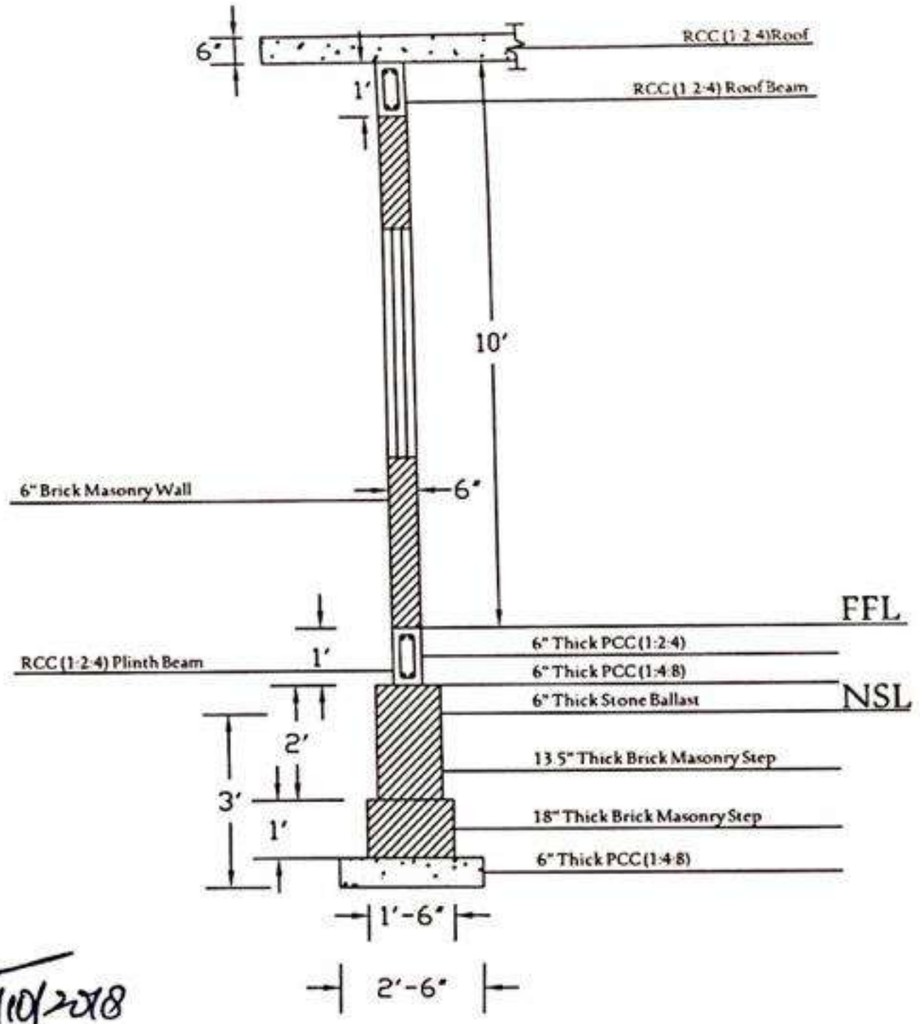
Brick Wall Section
