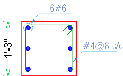
COLUMN C-1
