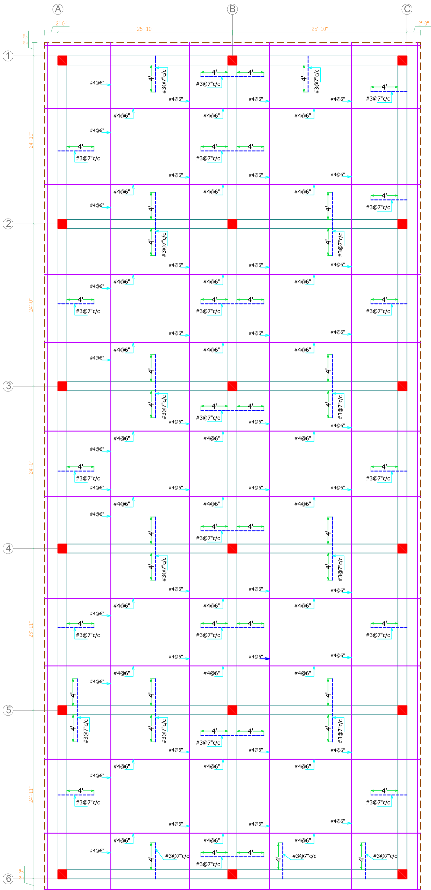
FIRST FLOOR SLAB REINFORCEMENT PLAN
