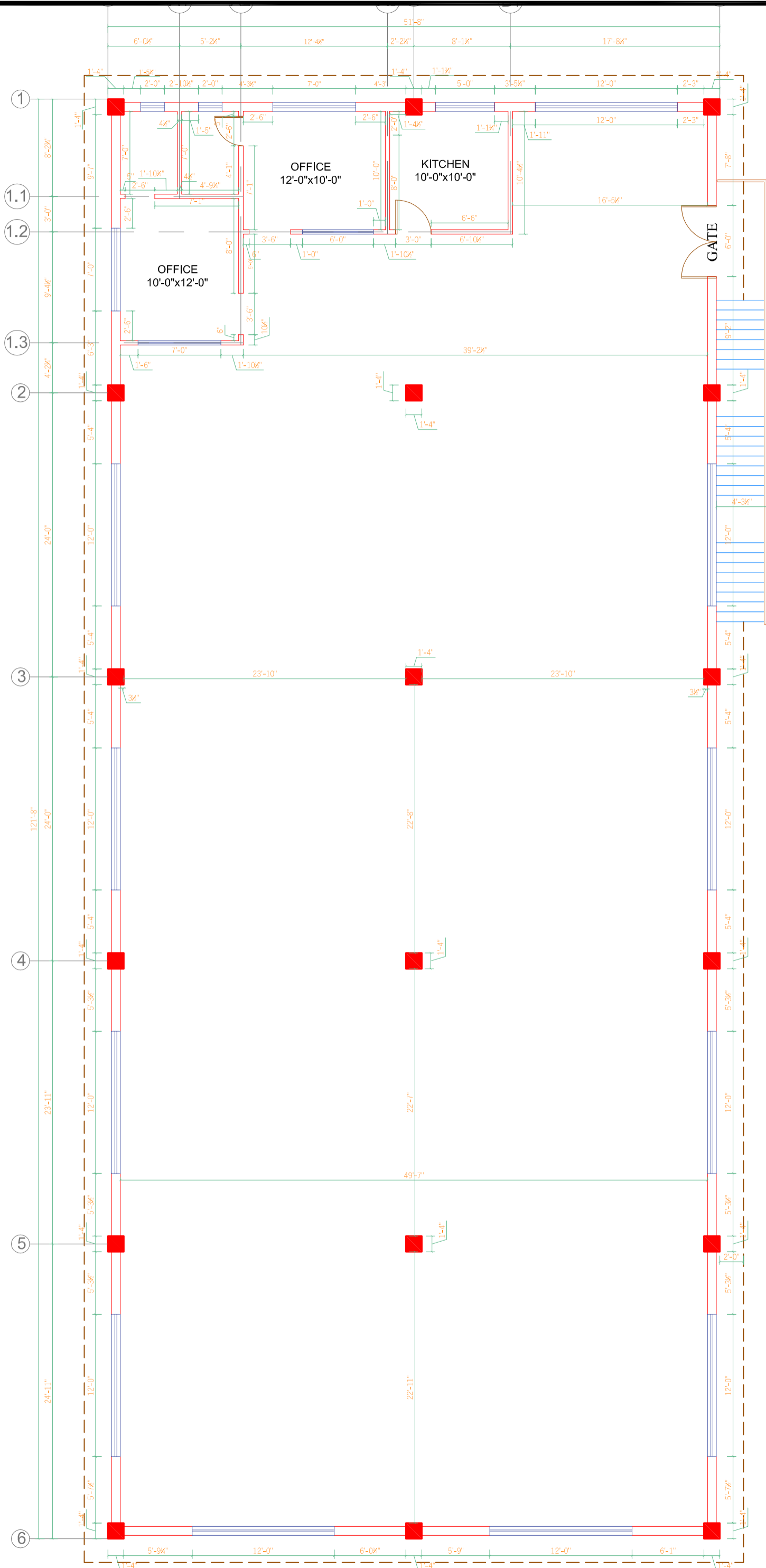
FIRST FLOOR DIMENSION PLAN
