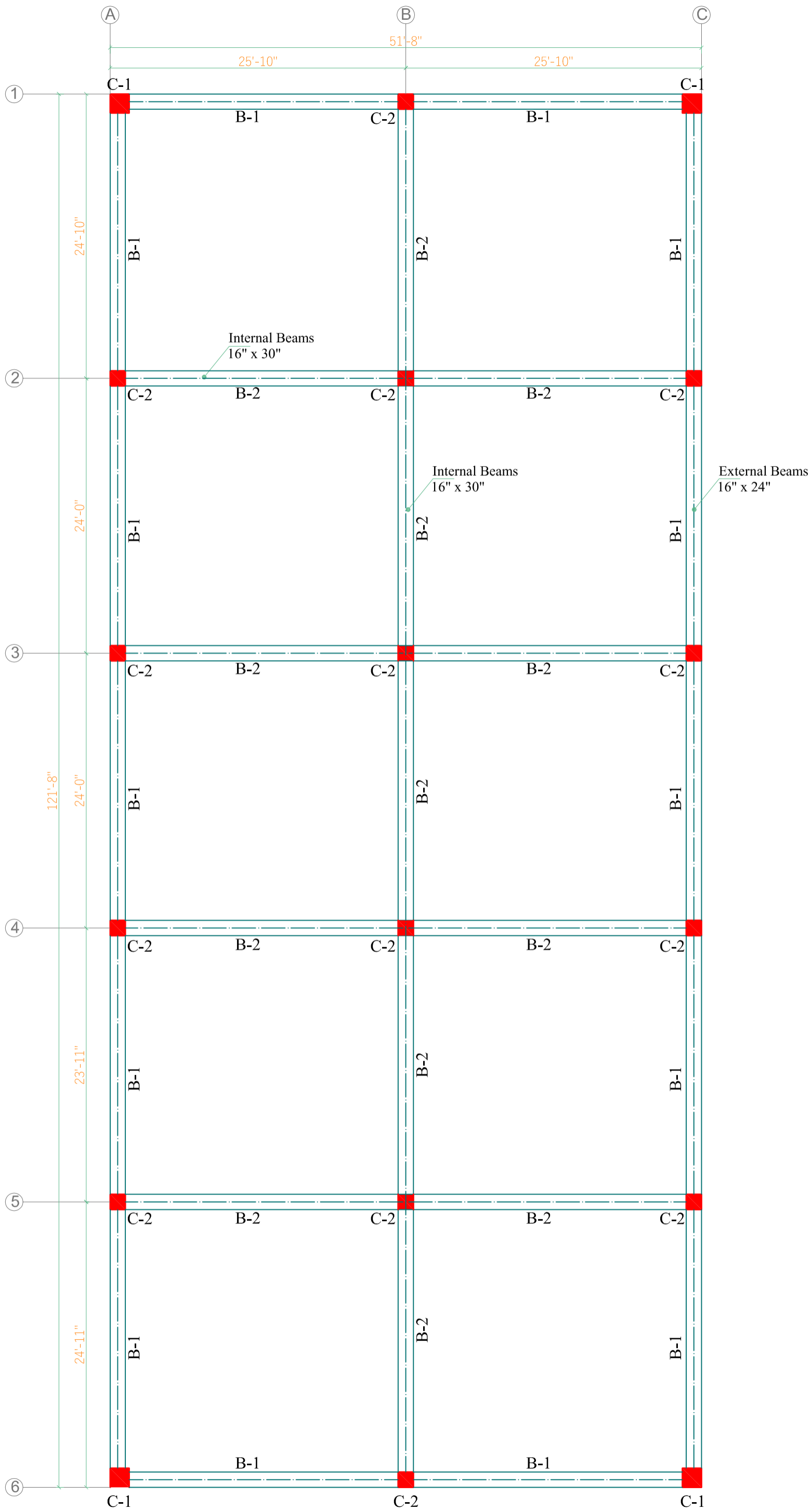
GROUND FLOOR COLUMN & BEAM LAYOUT PLAN
