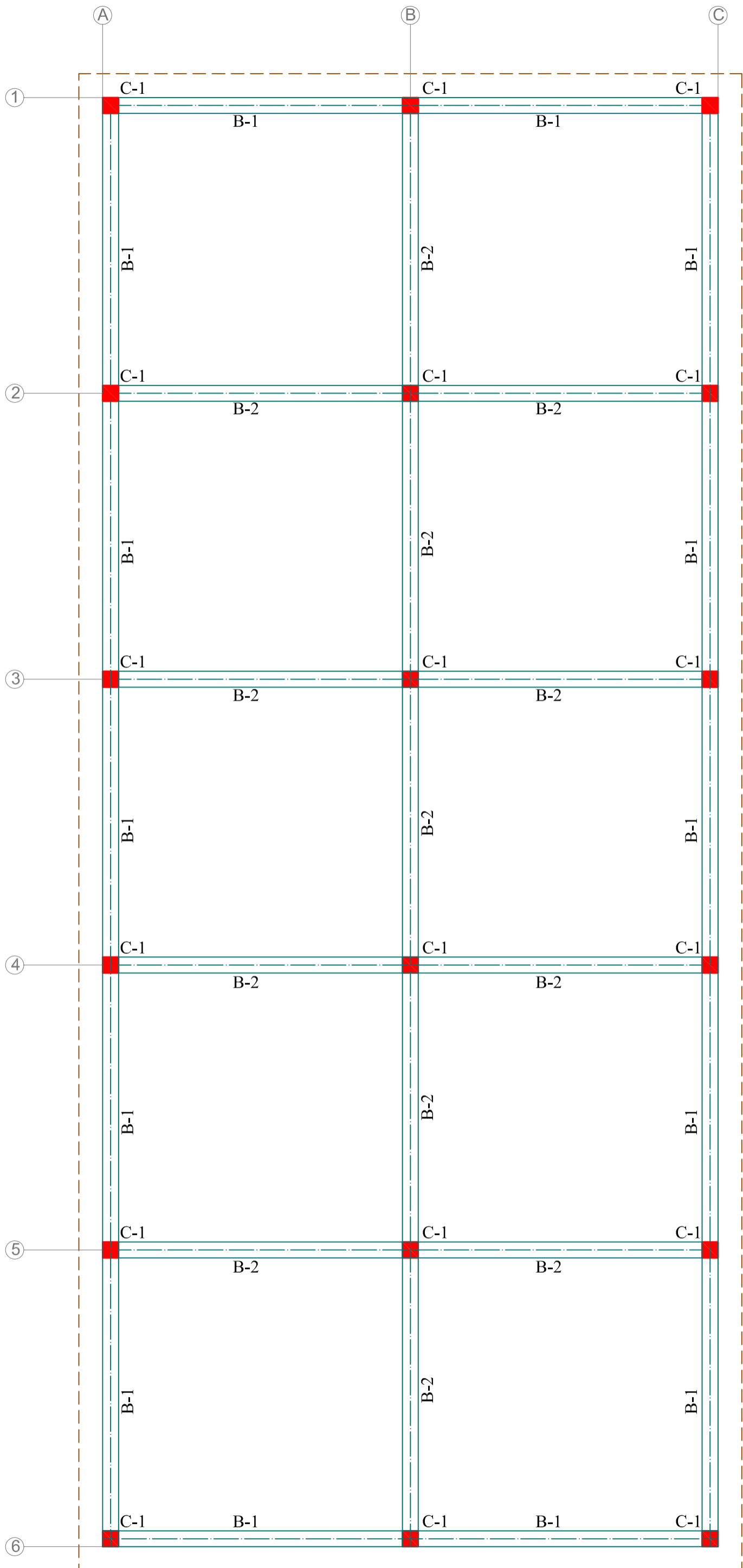
FIRST FLOOR COLUMN & BEAM PLAN
