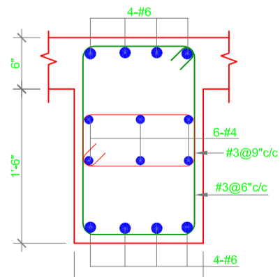
BEAM B-2
