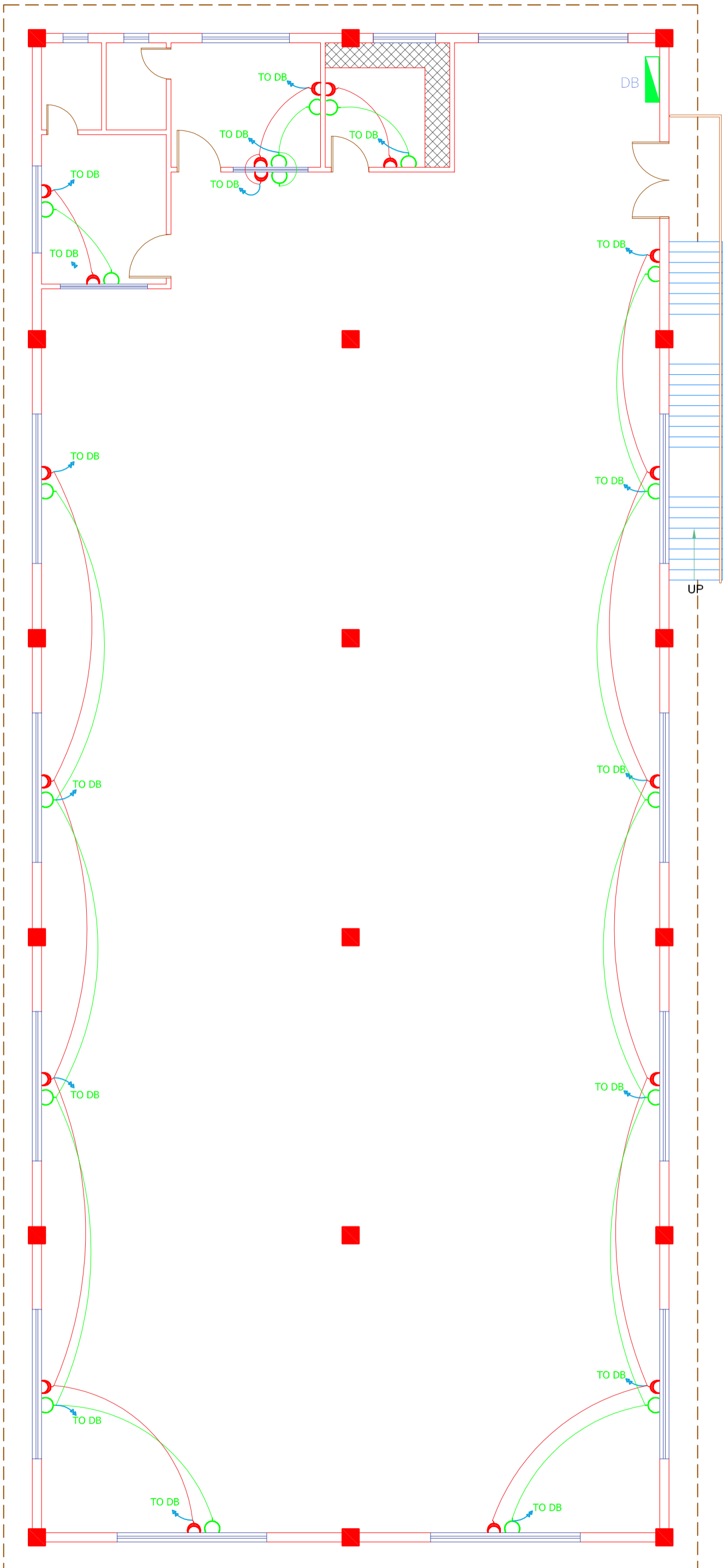
FIRST FLOOR POWER PLAN
