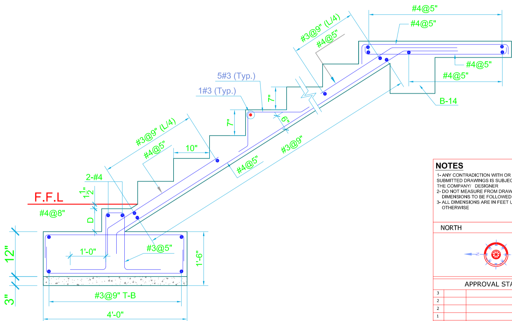
SIDE STAIR CASE DETAIL (FIRST FLIGHT)
