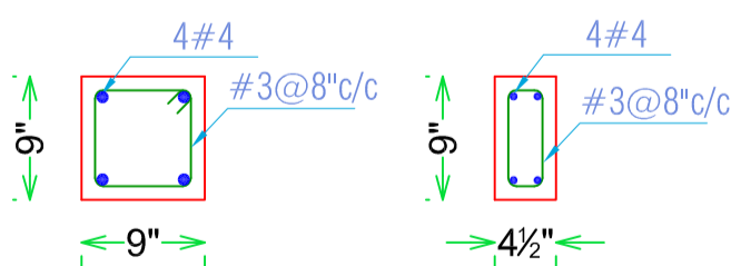
LINTEL BEAM
