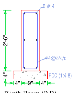
Plinth Beam (P.B)
