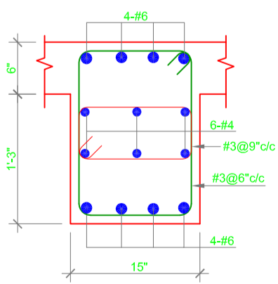
BEAM B-1
