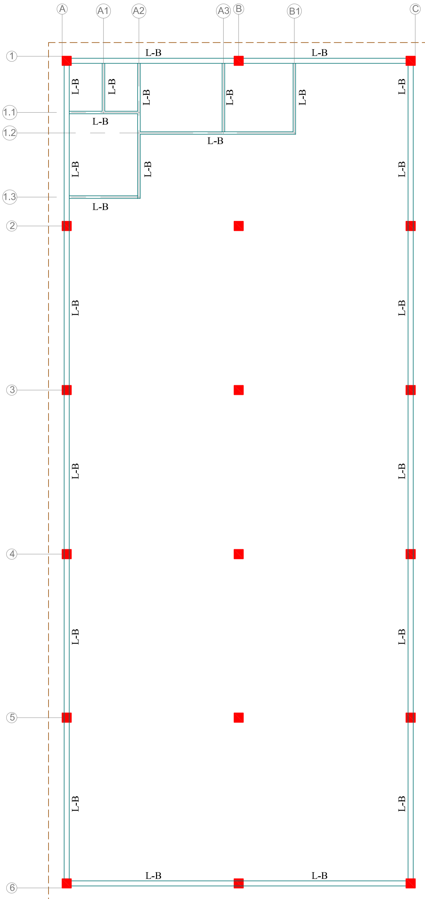
FIRST FLOOR LINTEL BEAM PLAN
