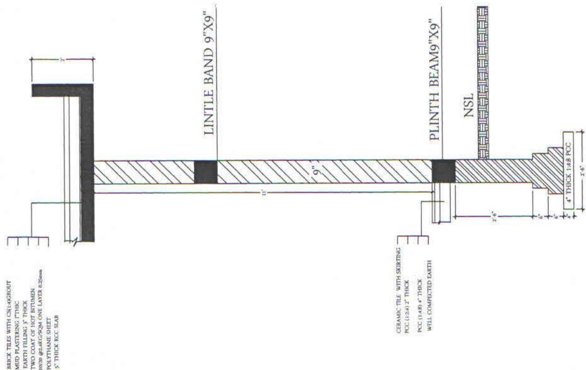
X-SEC OF ROOM WALLS
