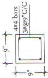
X-SEC OF PLINTH AND LINTLE BAND and Columns
