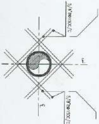
REINFORCEMENT DETAIL AROUND PIPE (SCALE - 1:30)
