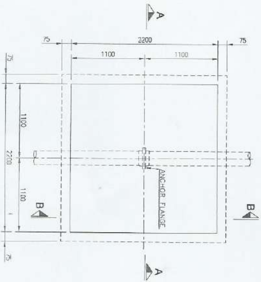
PLAN (SCALE - 1:30)
