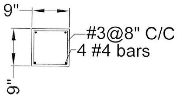
X-Section of Plinth and Lintel Beams
