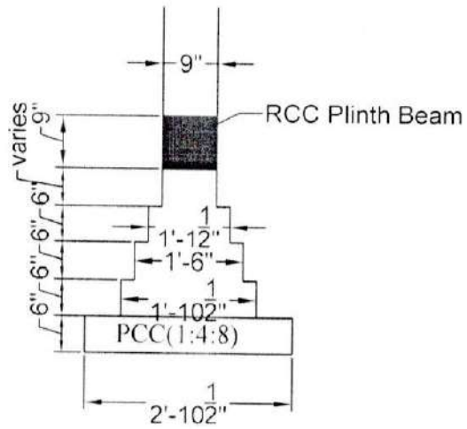
X-Section of Foundation
