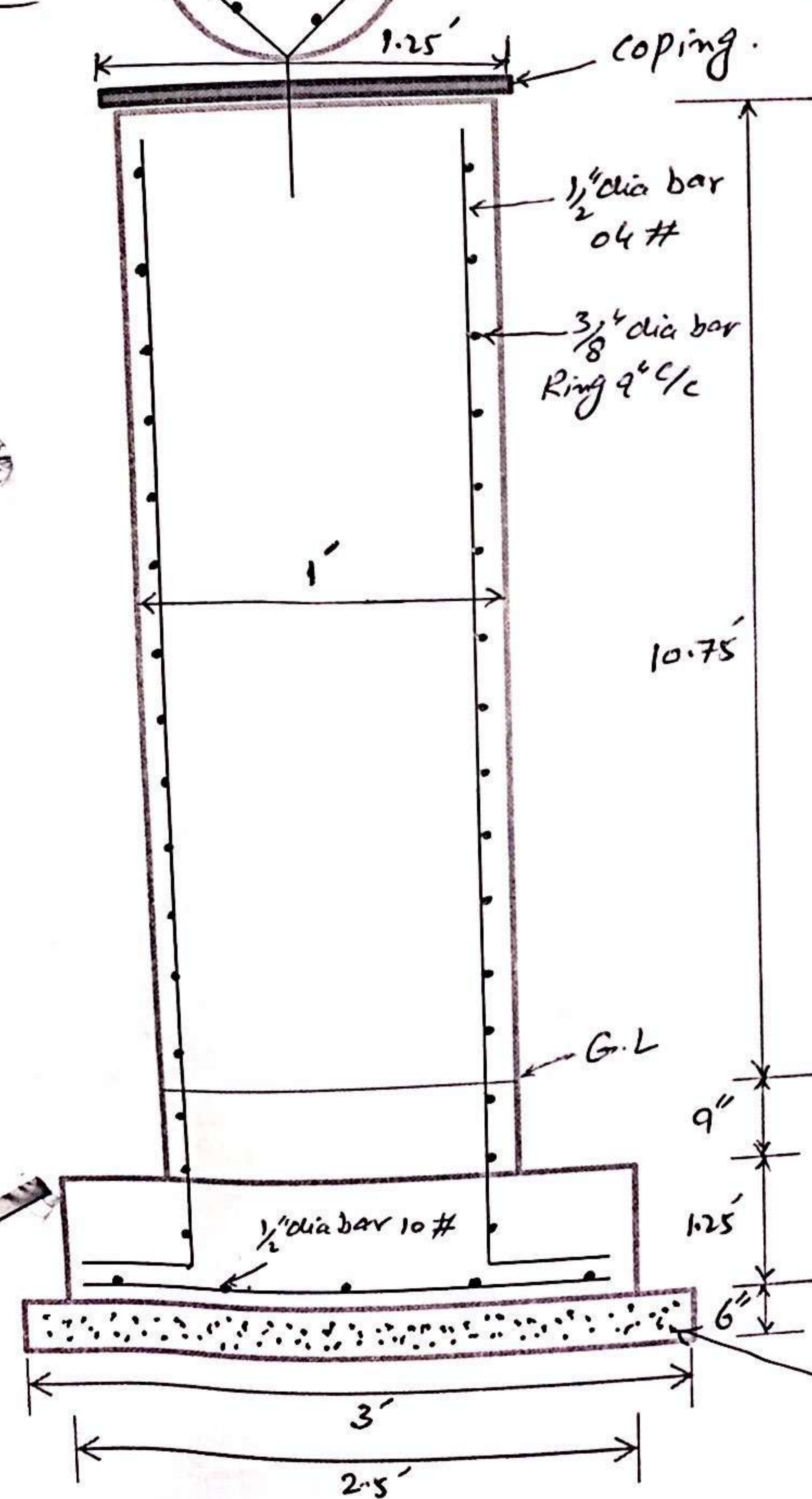
X-SECTION OF RCC COLUMN
