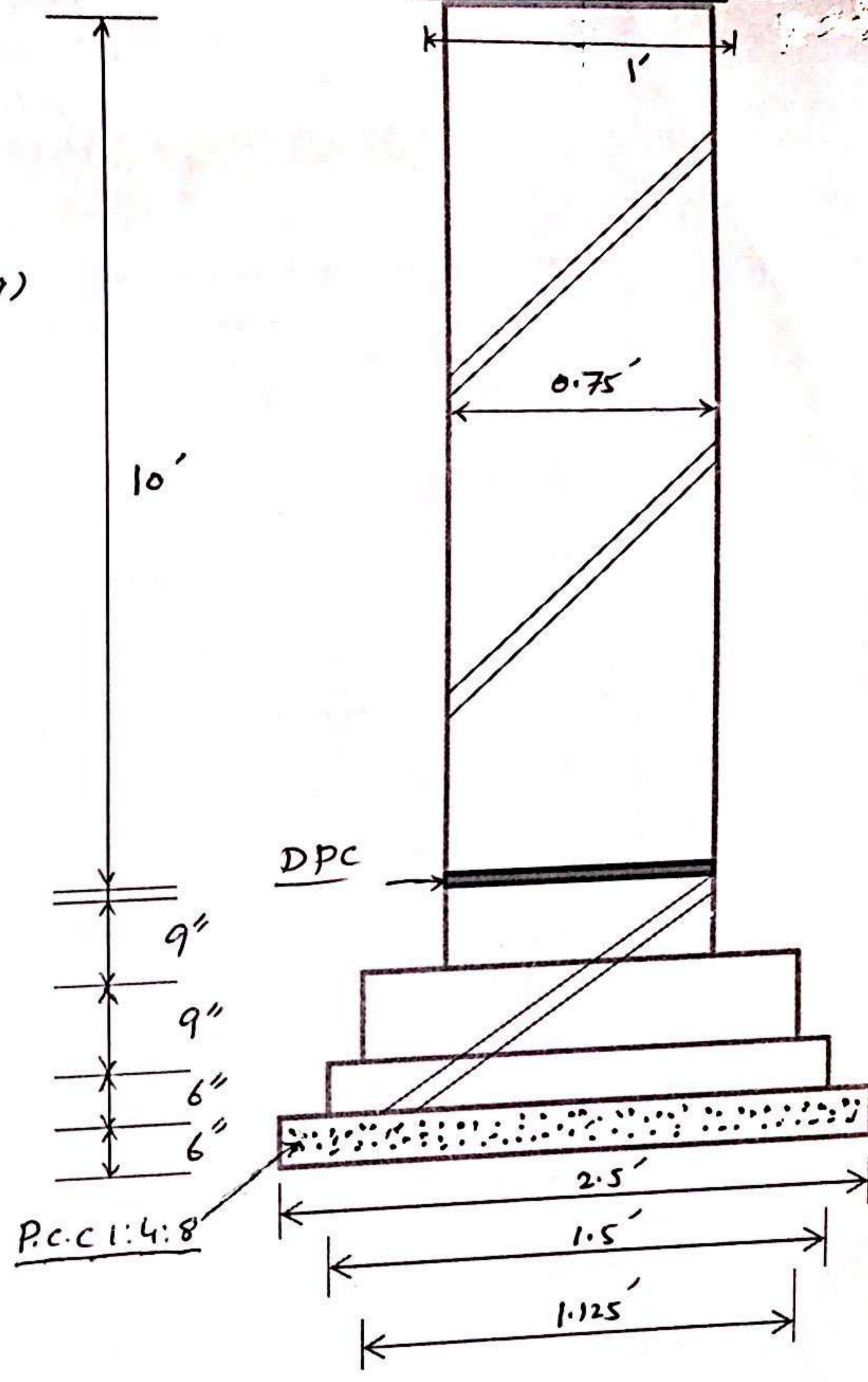
X-SECTION OF BRICK WALL
