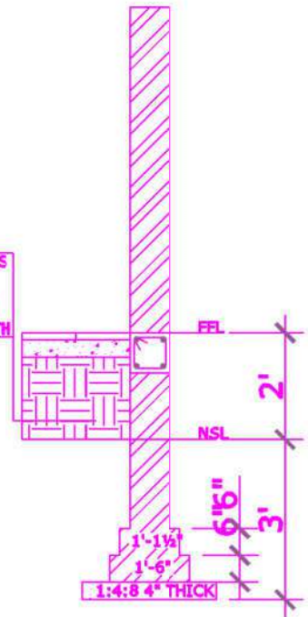
X-SEC OF 9" WALL
