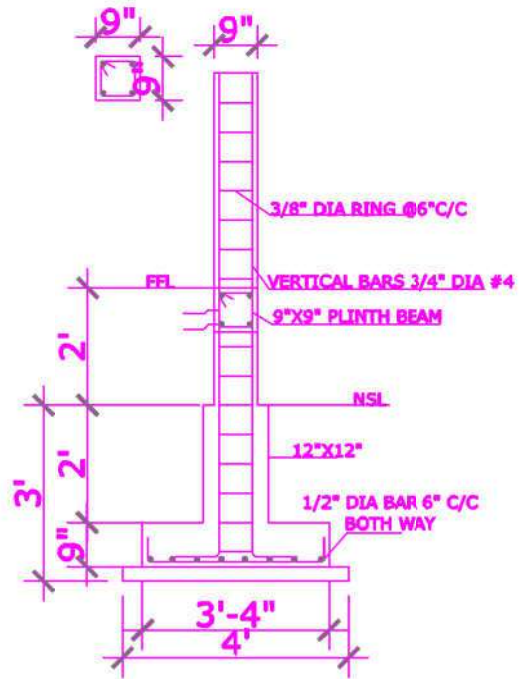
X-SEC OF 9"X9" COL
