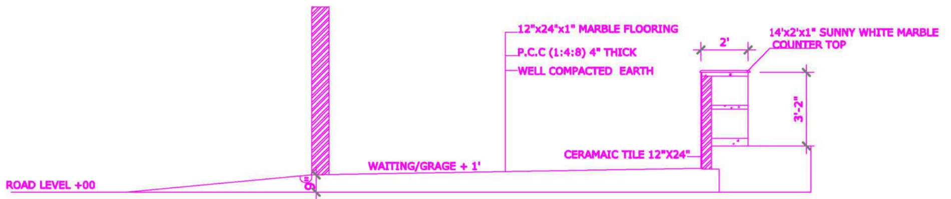
RAMP AND SERVICE COUNTER DETAIL
