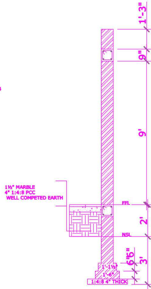
X-SEC OF 9" WALL
