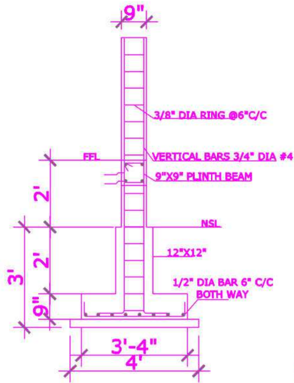
X-SEC OF 9"X9" COL
