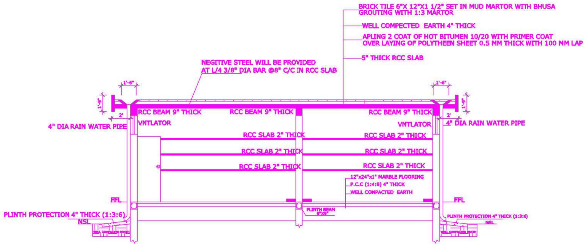
X-SECTION AT A-A
