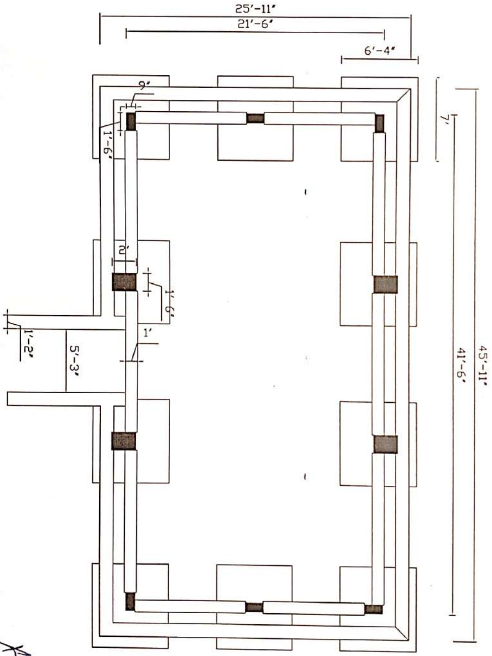
PLINTH LEVEL PLAN
