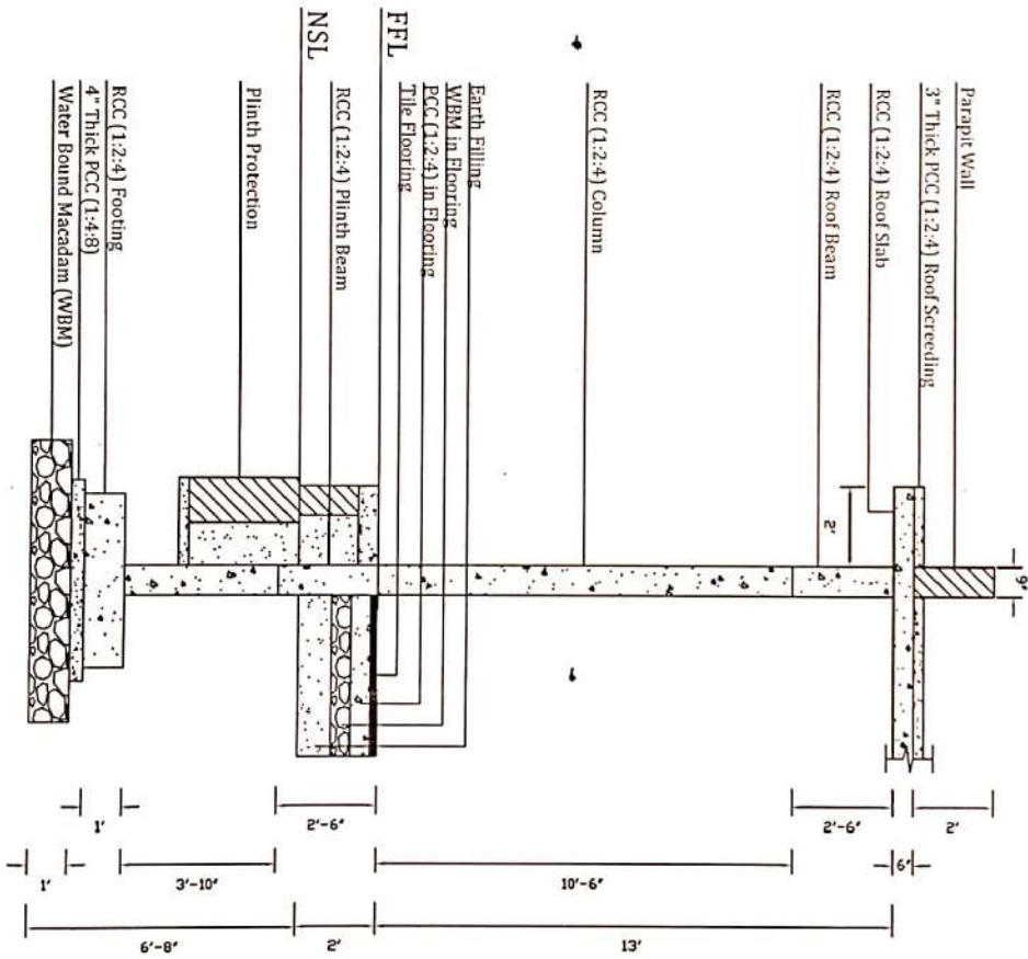
COLUMN SECTION
