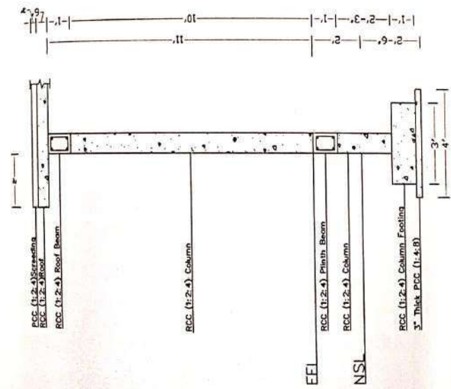
RCC Column Section
