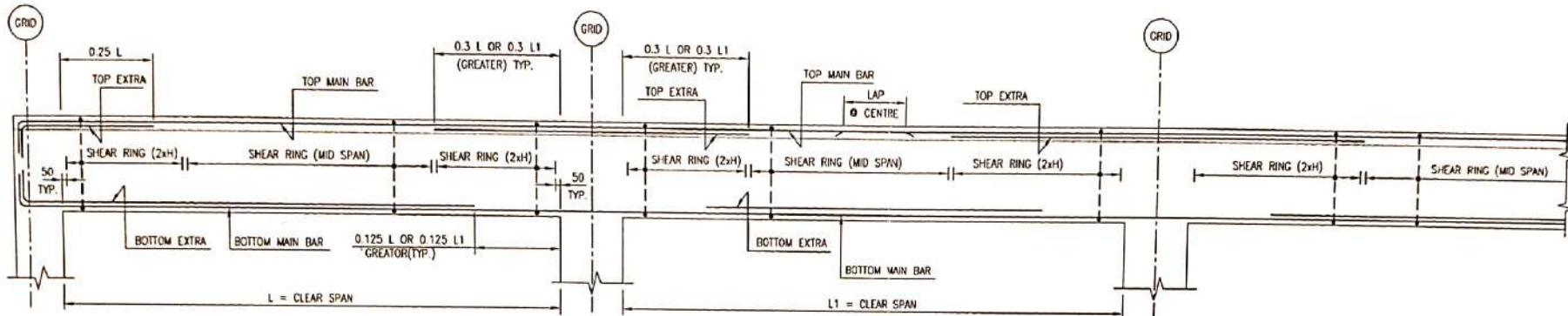
TYPICAL TOP SLAB BEAM SECTIONAL ELEVATION
