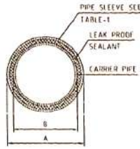
TYP. CROSS SEC. DETAILS OF PIPE FOR WALL OPENING (SCALE 1:10)
