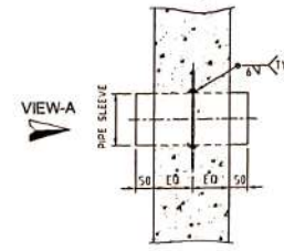
TYPICAL SLEEVE DETAIL (SCALE 1:10)
