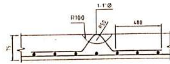
LIFTING HOOK DETAIL (SCALE 1:10)
