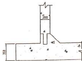
TYPICAL CONSTRUCTION JOINT (SCALE 1:20)
