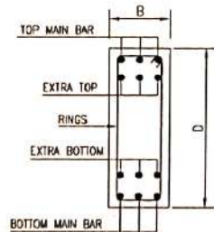
BEAM CROSS SECTIONAL DETAIL
