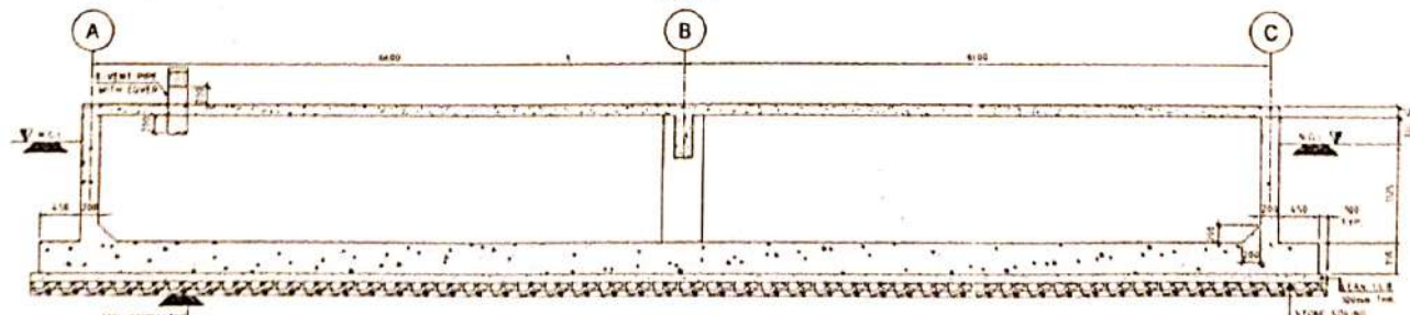
SECTION B-B (SCALE 1/8)
