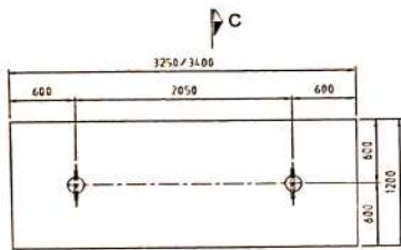
TYPICAL PORTABLE SLAB DETAIL (SCALE 1:25)
