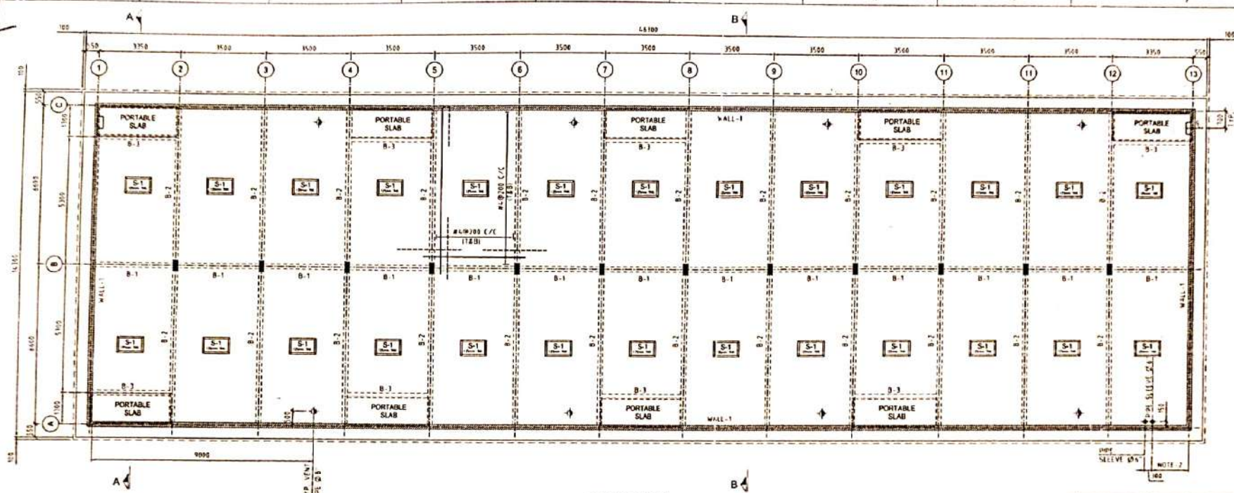
TOP SLAB PLAN (SCALE 1/8)
