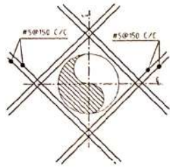
TYP. REINFORCEMENT DETAIL AROUND PIPE SLEEVE (SCALE 1:10)
