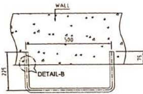
RUNGS DETAIL (SCALE 1:10)
