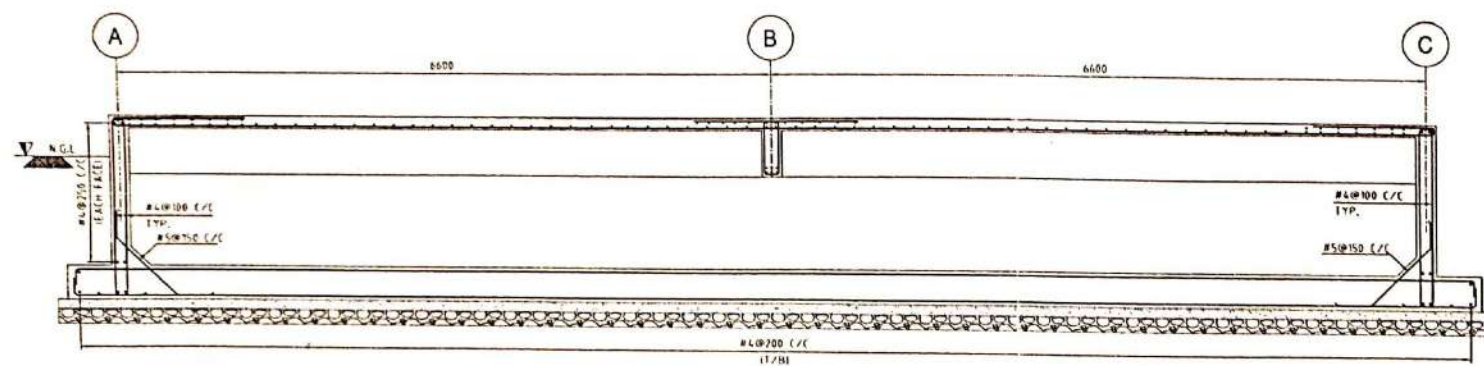
REINFORCEMENT SECTION SCALE 1/25
