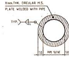
VIEW-A (SCALE 1:10)
