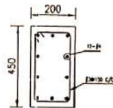
COLUMN (C-1) CROSS SECTIONAL DETAIL
