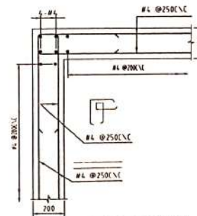
CORNER REINFORCEMENT DETAIL (SCALE 1:15)
