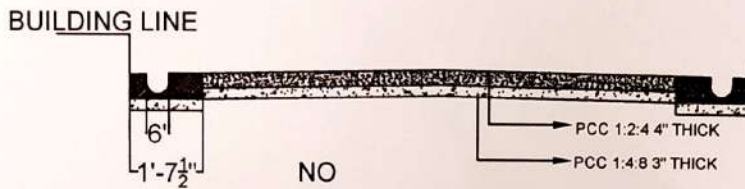
X-SEC OF 12' WIDE PCC ROAD ALONG STREET DRAIN
