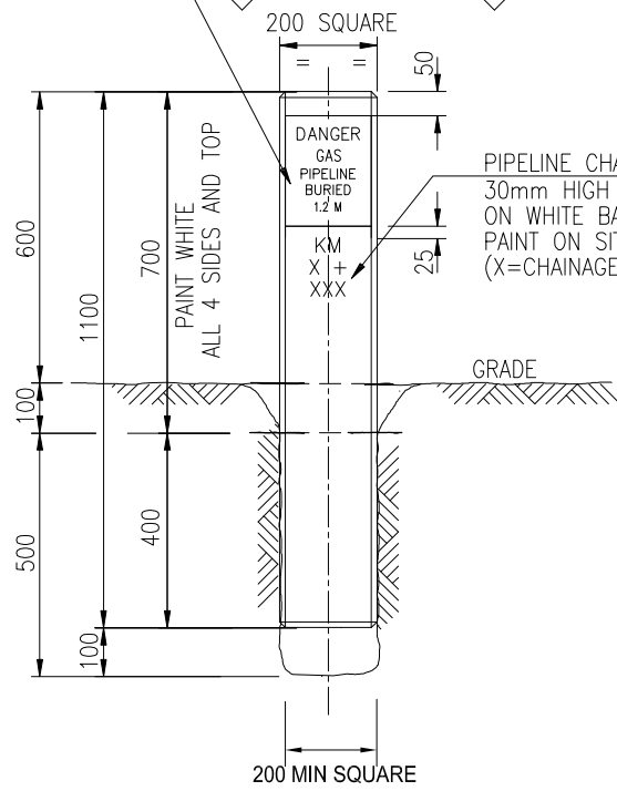
ELEVATION - FRONT SIDE MARKER POST LOOKING IN DIRECTION OF PIPELINE FLOW
