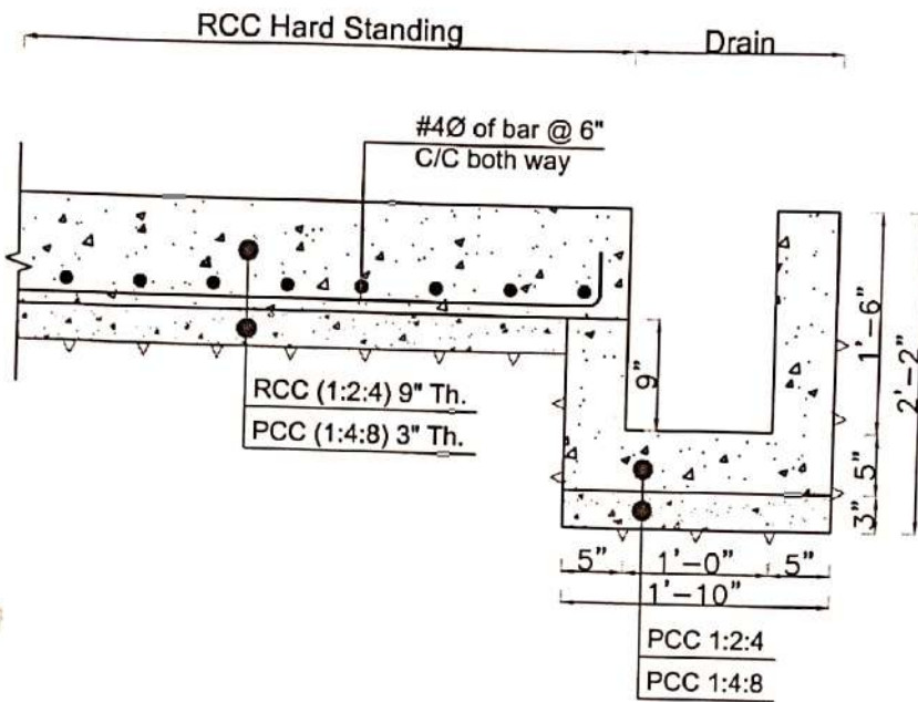
a) Cross Section of RCC Hard Standing with PCC Drain
