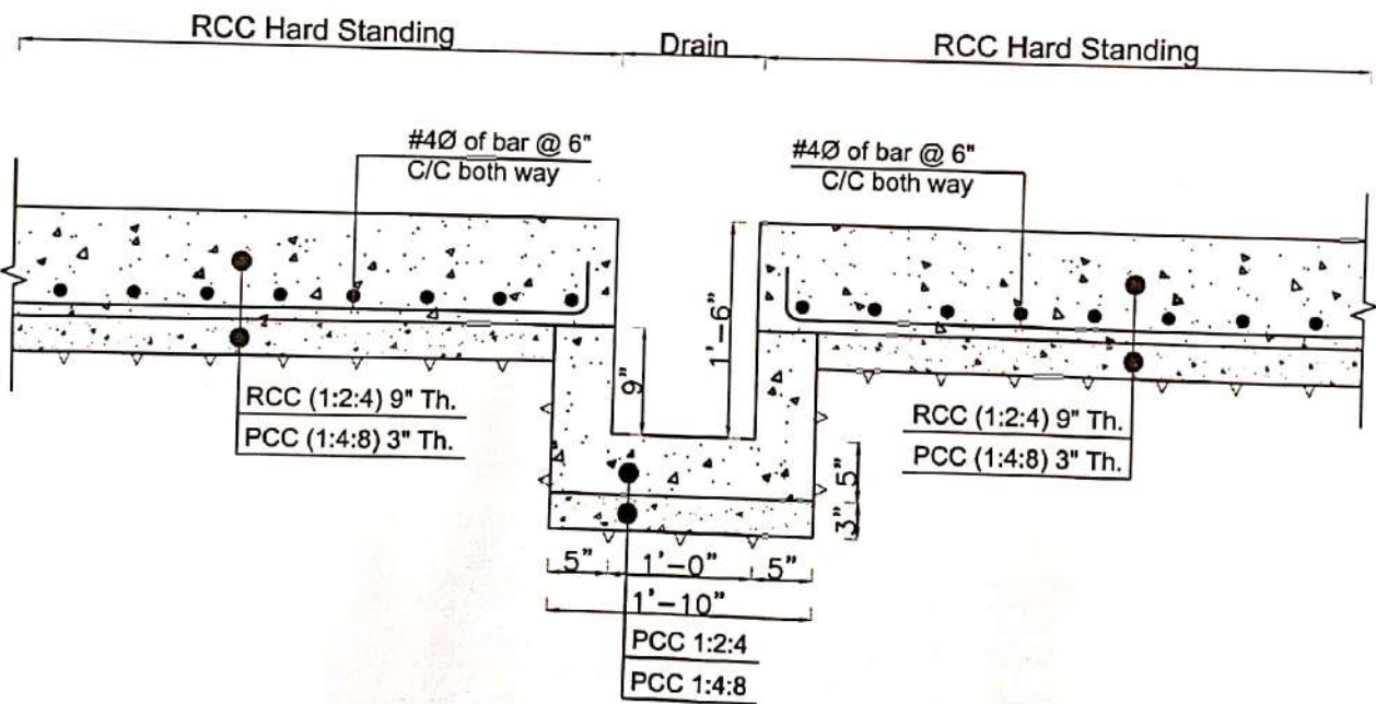
b) Cross Section of RCC Hard Standing with PCC Drain
