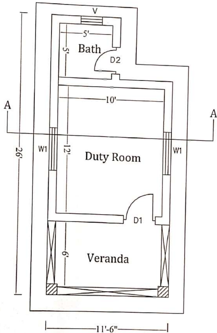
Room Plan
