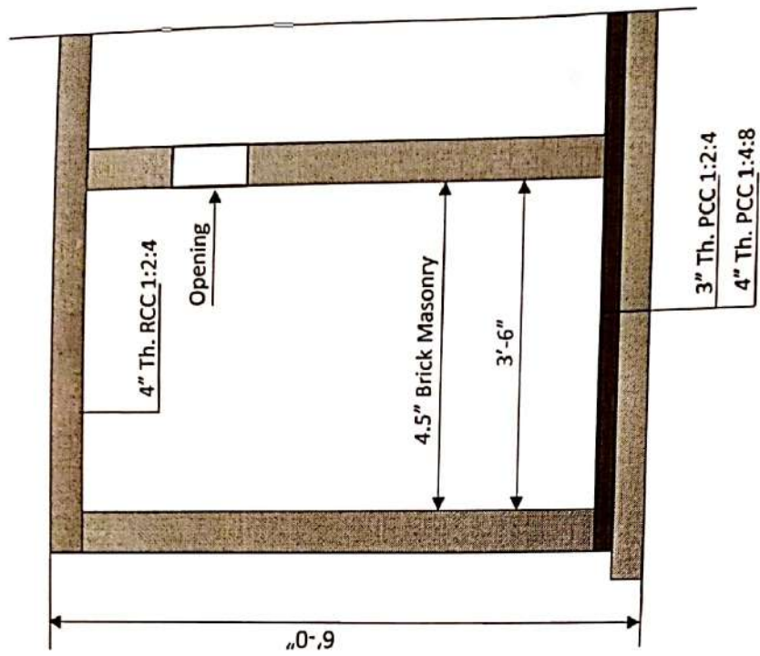
Typical Section of Septic Tank
