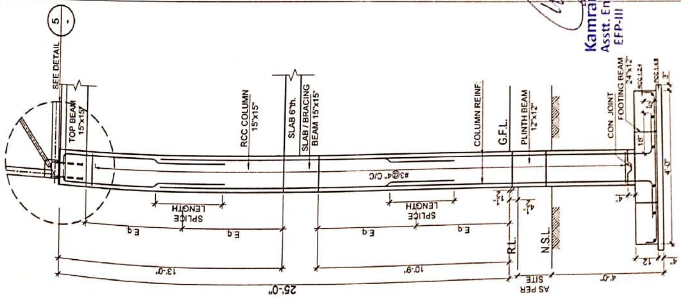
SECTION A-A OF (F2) FOOTING & COLUMN SECTION
