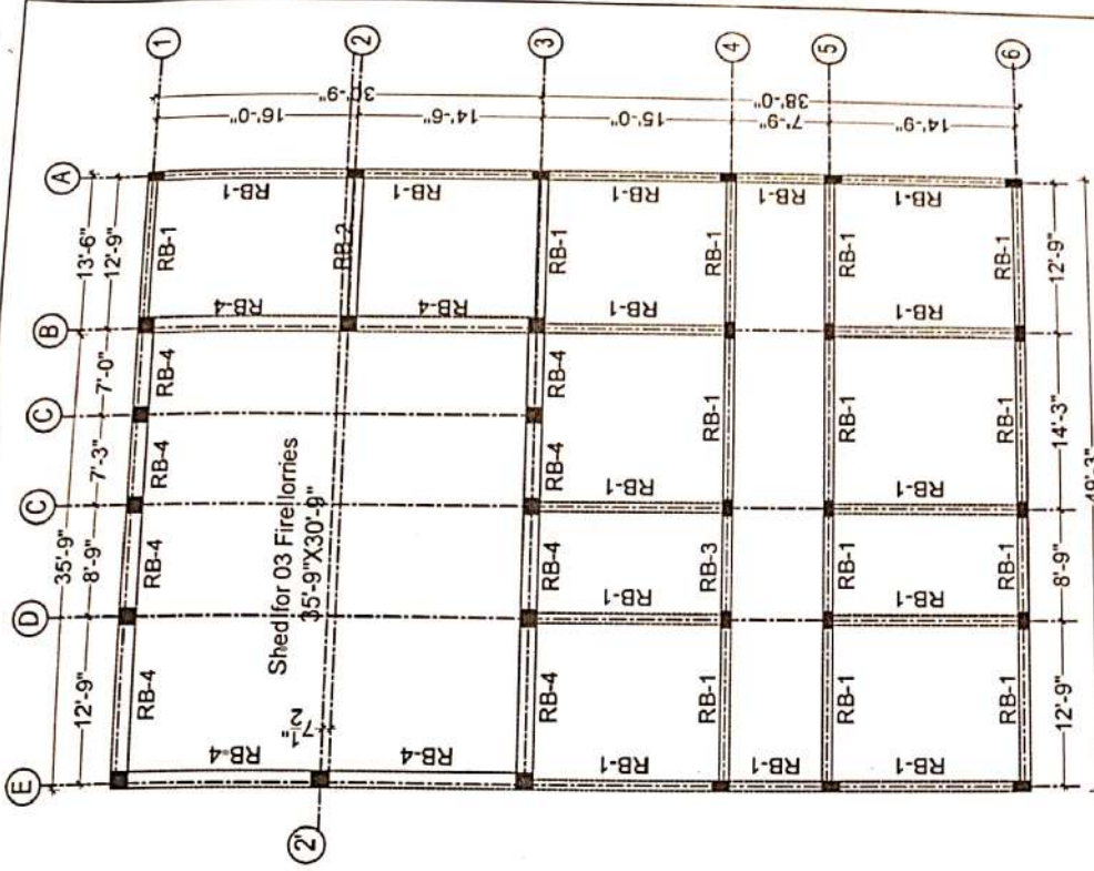
ROOF BEAMS FRAMING PLAN
