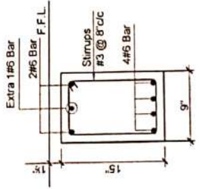
Plinth Beam PB-1
