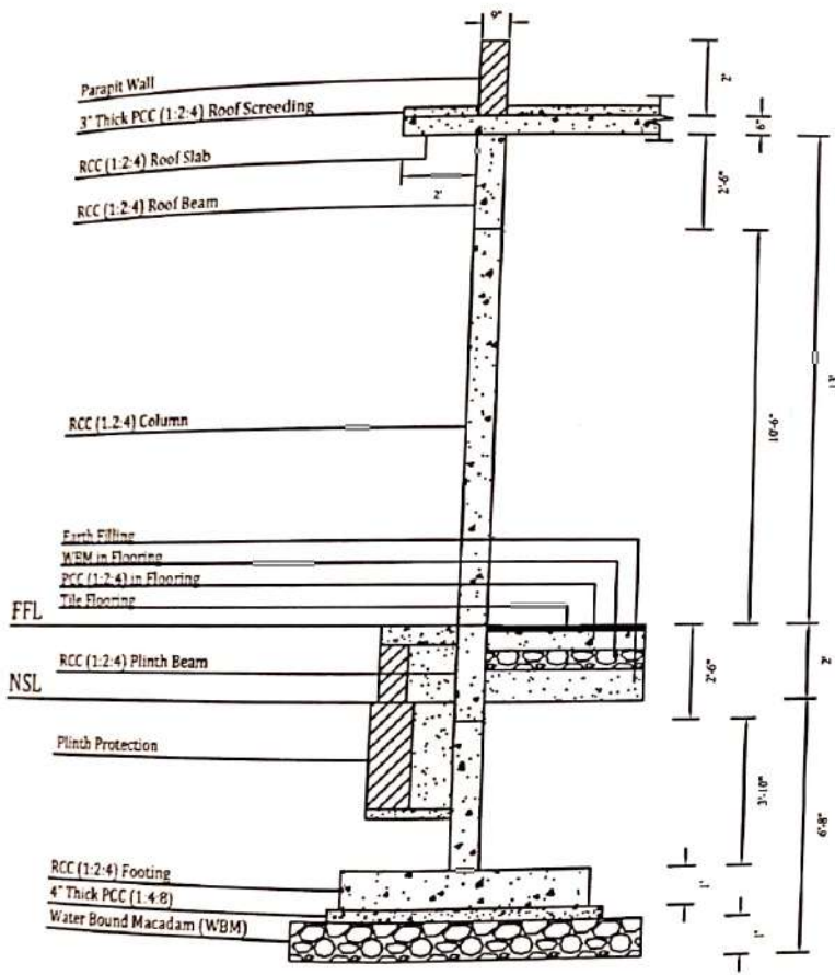
COLUMN SECTION
