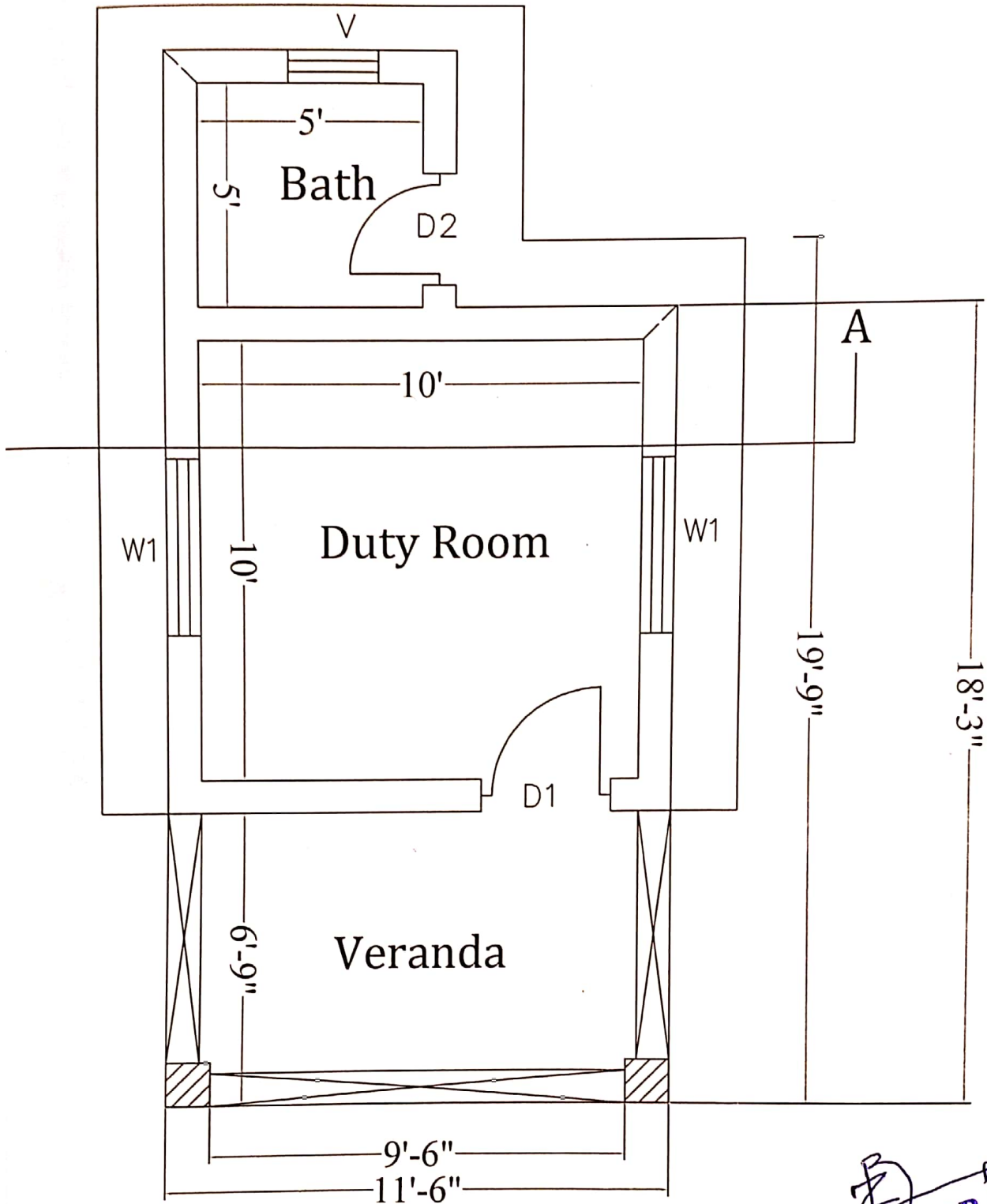
Room Plan
