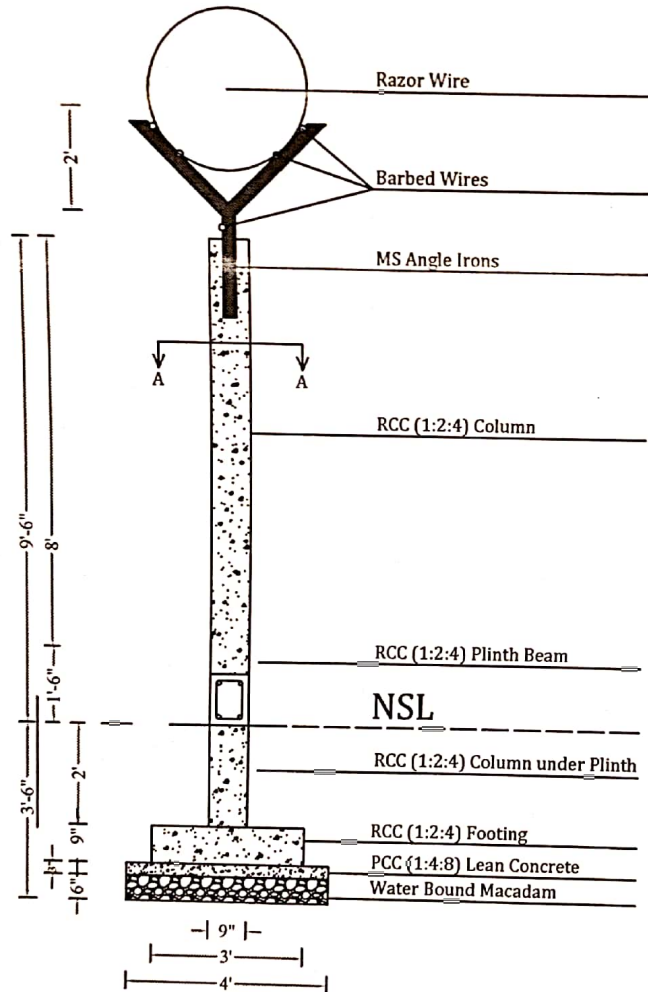
Column Section
