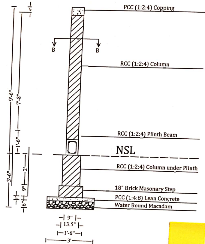
Wall Section
