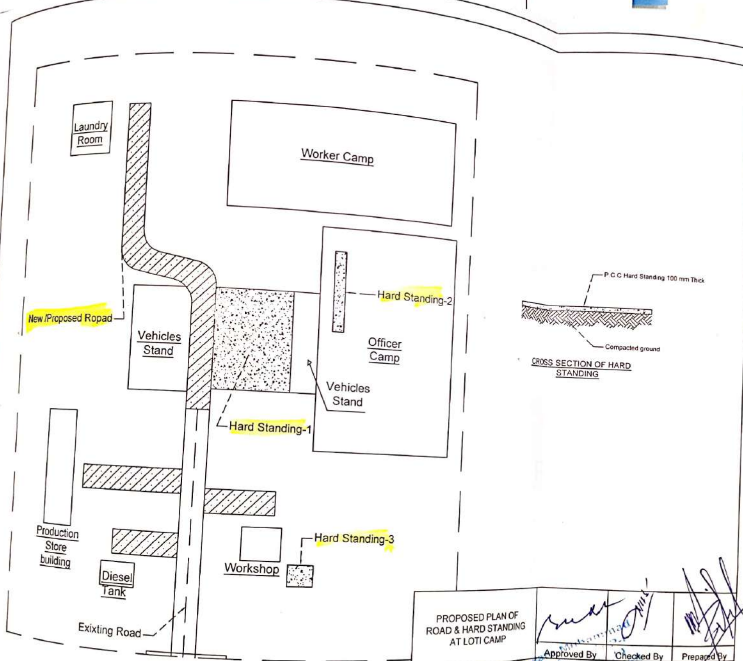
PROPOSED PLAN OF ROAD & HARD STANDING AT LOTI CAMP
