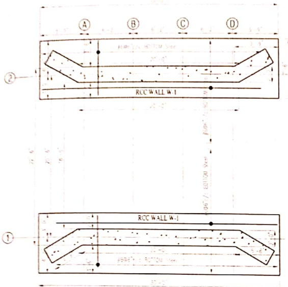
FOUNDATION LAYOUT PLAN SCALE: 3/16"=1'-0"
