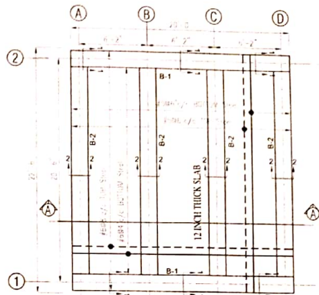
ROOF BEAM FRAMING PLAN SCALE: 3/16"=1'-0"
