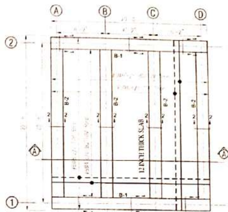
ROOF BEAM FRAMING PLAN SCALE: 1/16"=1'-0"
