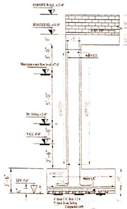
TYP. ELEVATION OF RCC WALL W-1
