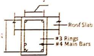
CENTER WALL ROOF BEAM
