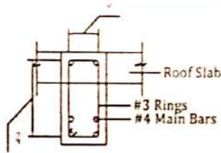
ROOF BEAM
