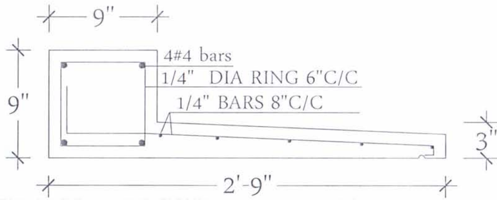
X-SEC OF SUN SHADE OVER WINDOWS DOORS
