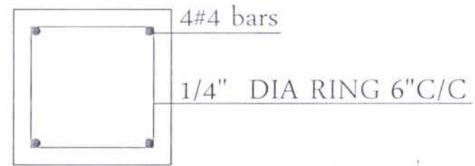
X-SEC OF LINTLE BAND
