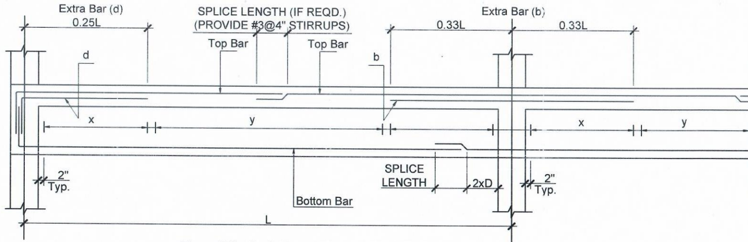
Typ. Plinth & Roof Beam Reinf. detail
