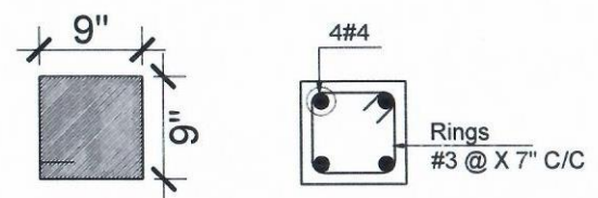
COLUMN (C1)
