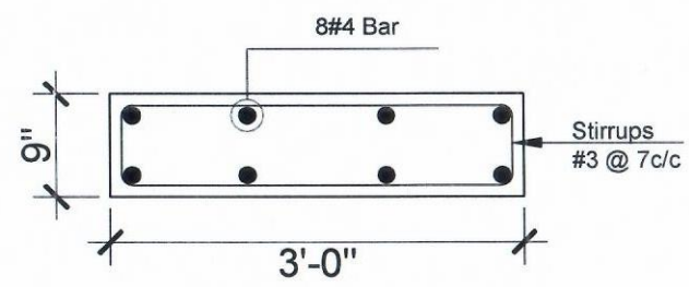
Footing Beam
