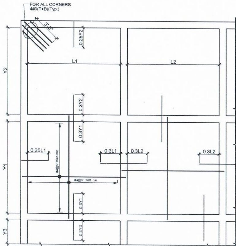
Typ. SLAB REINFORCEMENT (CUT OFF POINTS)
