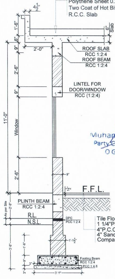
WALL & FOOTING SEC.
