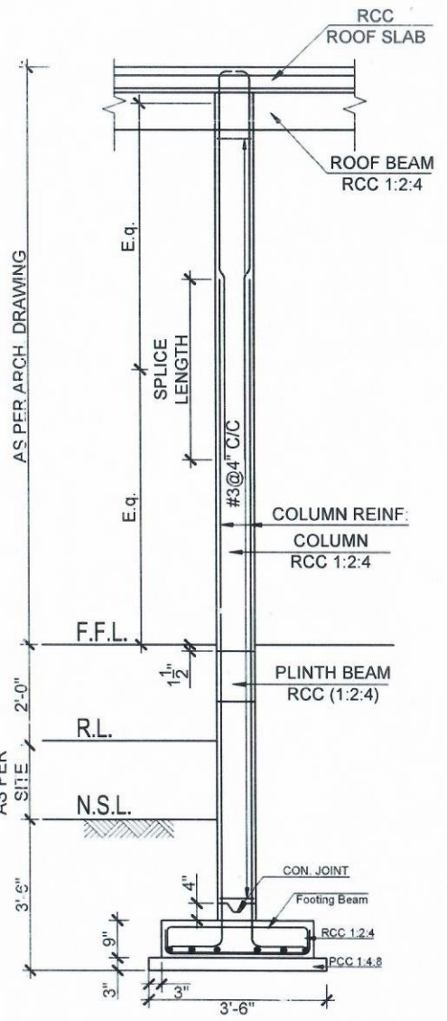
SECTION A-A (F1) FOOTING & COLUMN SECTION
