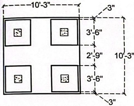
FOUNDATION PLAN
