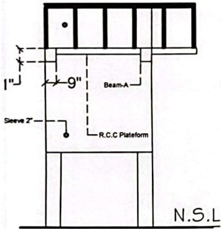
X-SECTION B-B
