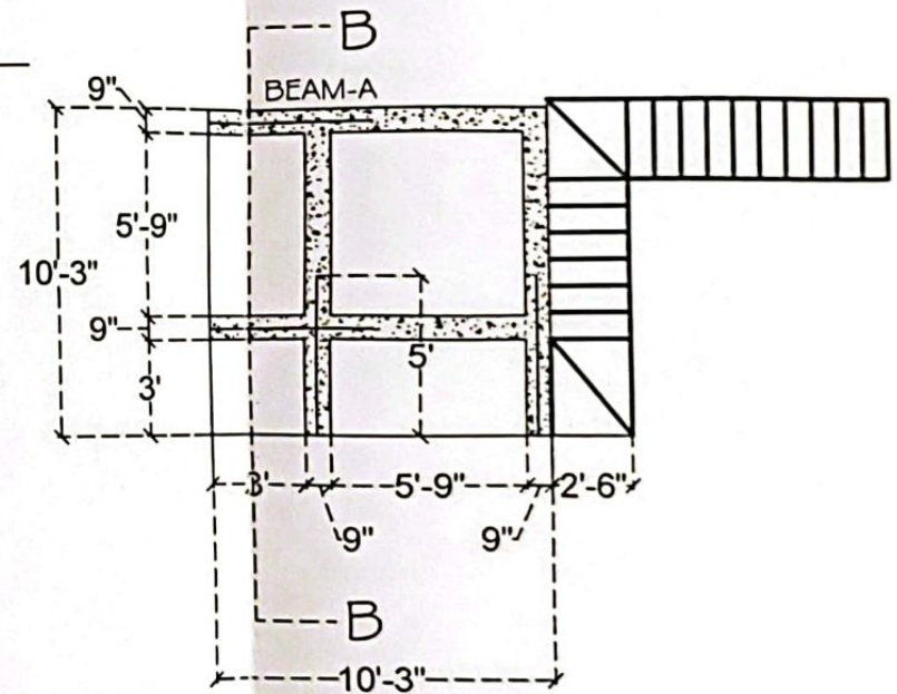
R.C.C PLATFORM
