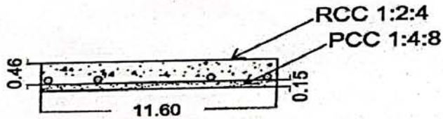
Section BB Mud Pump Foundation
