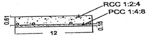
Section CC Main Foundation
