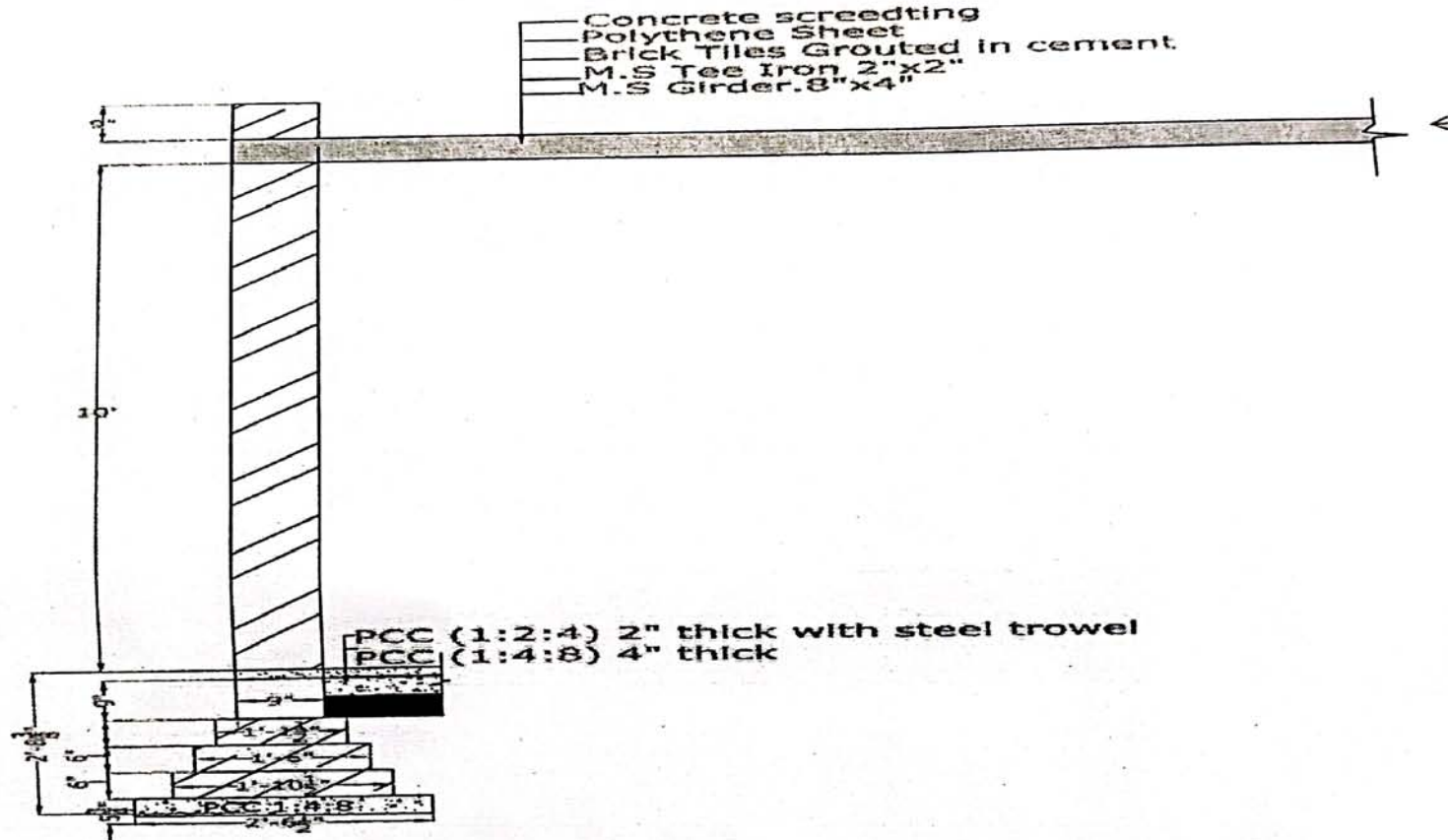
X-Section of Kitchens & Baths Walls
