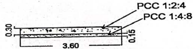
Section DD Mud Tanks Foundation
