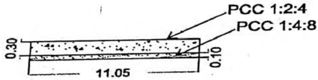
Section AA Generator Foundation
