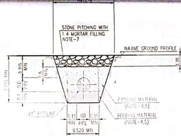
STANDARD DETAIL 8" PIPELINE TRENCH TYPE-B
