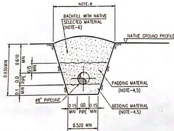
STANDARD DETAIL 8" PIPELINE TRENCH TYPE-C
