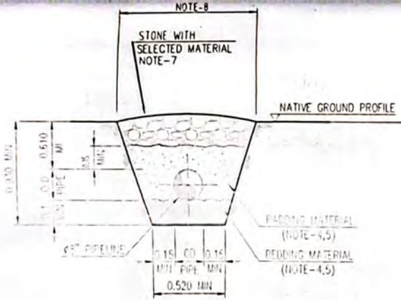
STANDARD DETAIL 8" PIPELINE TRENCH TYPE-A
