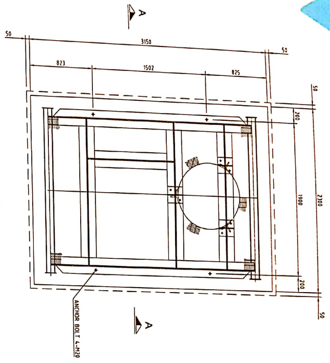
PLAN F-01A SCALE 1:30
