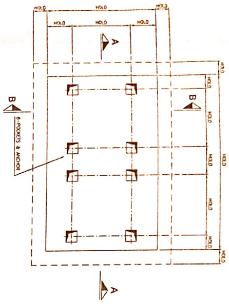
FOUNDATION PLAN OF (P-2510 B & P-2510 A)
