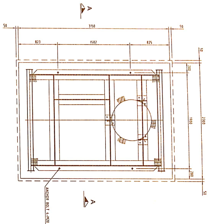
PLAN F-02 SCALE 1:30
