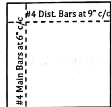
Room Roof Slab
