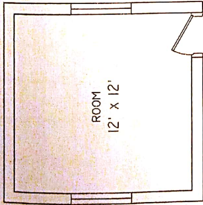
GROUND FLOOR ROOM PLAN
