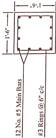
Column
