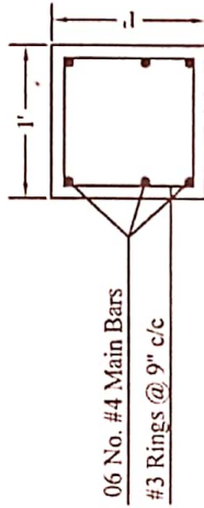
Plinth Beam
