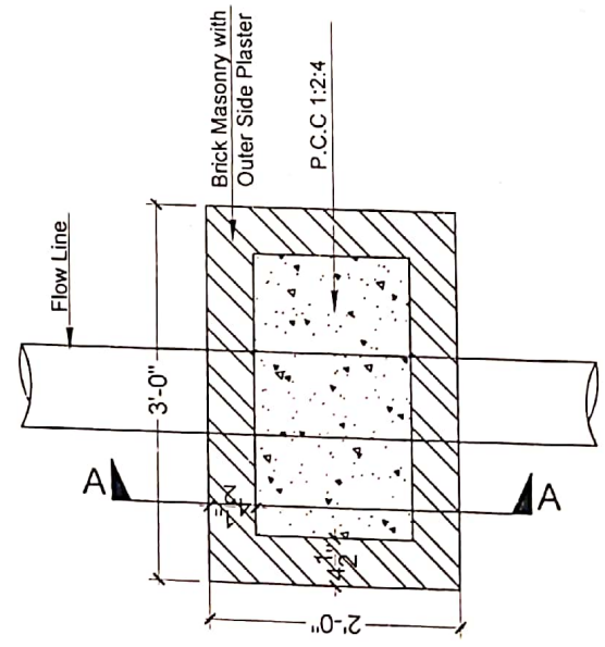
PIPE SUPPORT (WHA) PLAN
