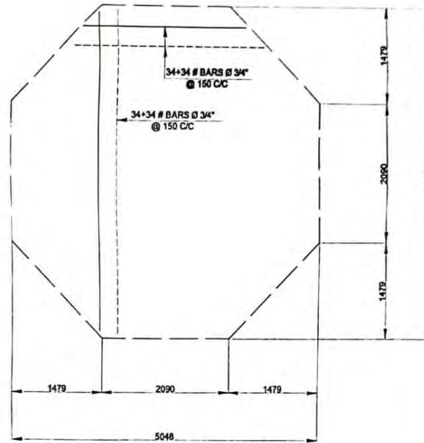
REINFORCEMENT PLAN
