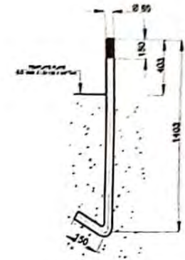
ANCHOR BOLT ARRANGEMENT
