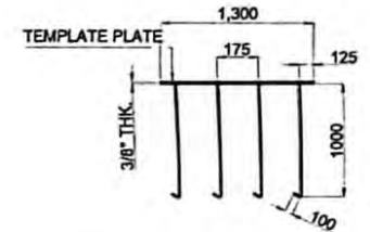
DEADMAN ANCHOR Ø 3/4" Qty= 8 Nos.FOR 1# PLATE
