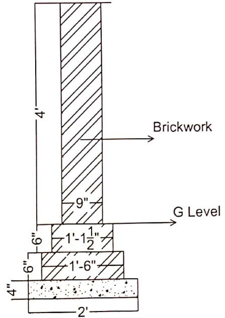
X-Section Dyke Wall Foundation
