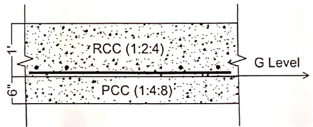
X-Section Separator Foundation
