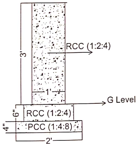
X-Section Pipe Sleepers Foundation
