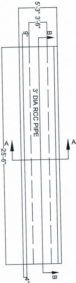
PLAN OF 3'-0" DIA RCC PIPE CULVERT
