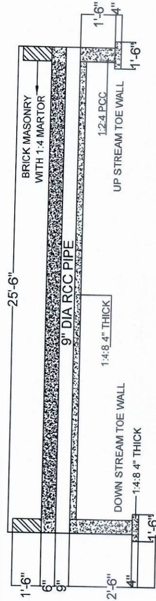
L-SECTION B - B 9" DIA RCC PIPE CULVERT
