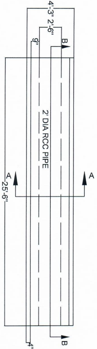
PLAN OF 2'-0" DIA RCC PIPE CULVERT
