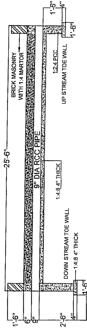
L-SEC AT B - B 9" DIA RCC PIPE CULVERT
