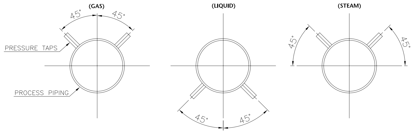
PROCESS PRESSURE TAP ANGLE (FOR HORIZONTAL PIPING)
