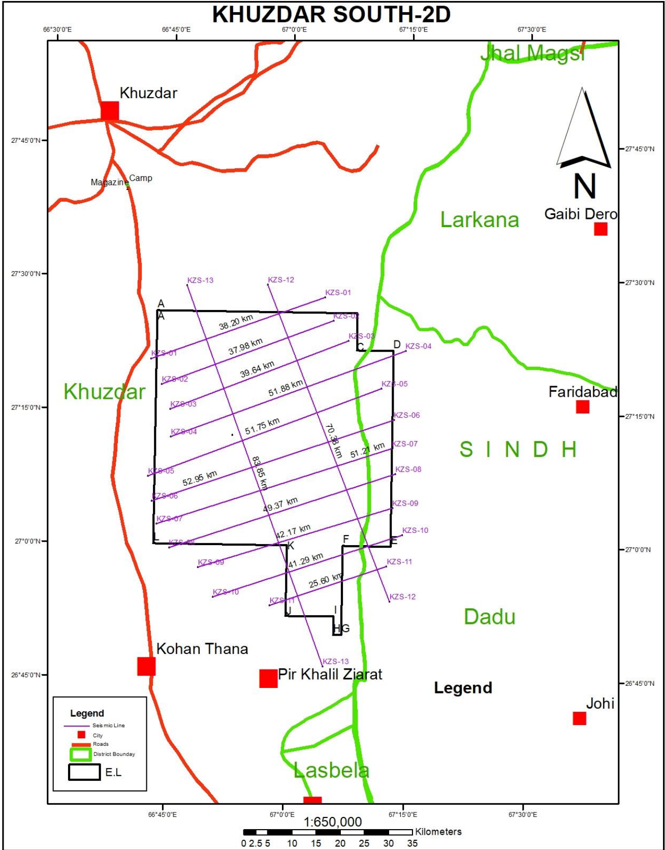
Seismic Base Map of Designed 2D Seismic acquisition program
