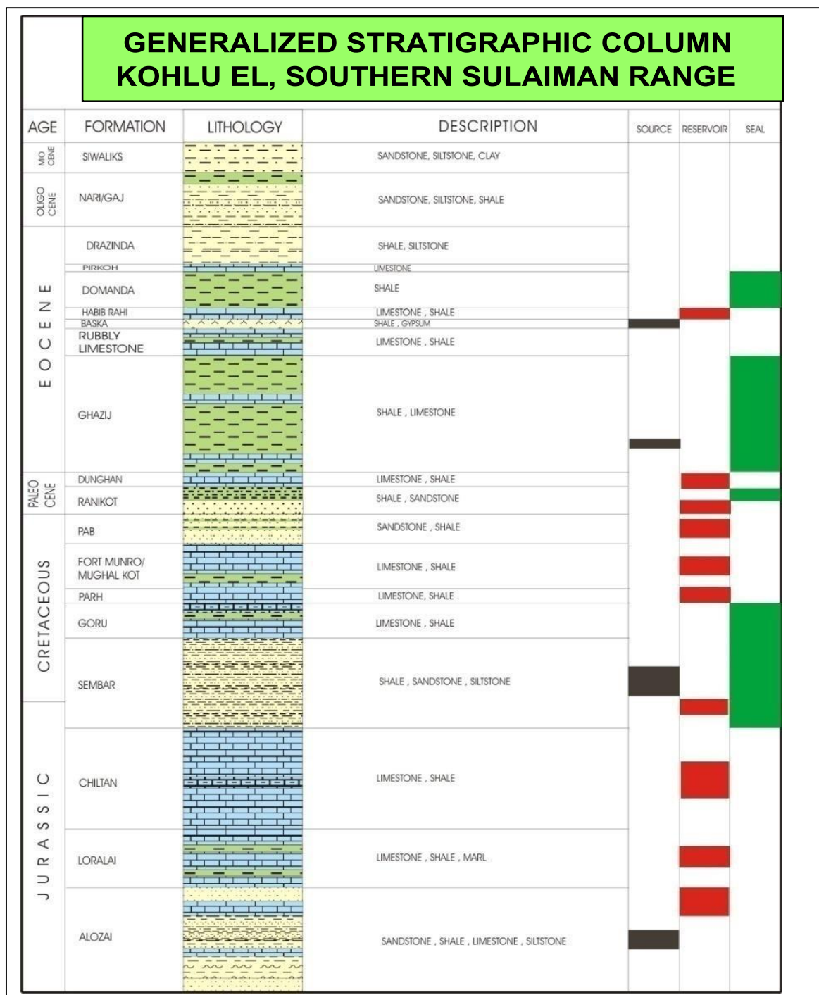
Figure-05: Generalized stratigraphic column of Kohlu block
