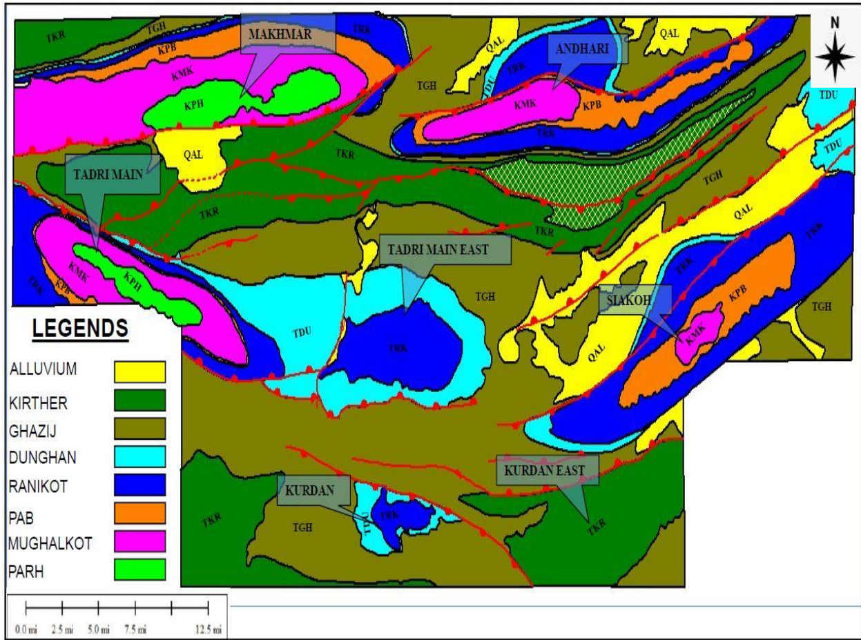
Figure-03: Structural style of Kohlu block
