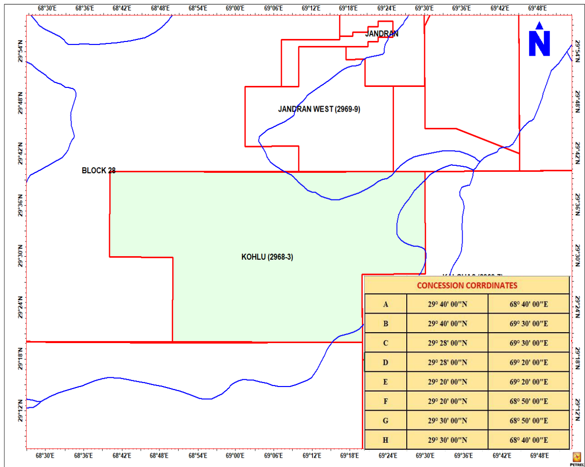
Figure-01: Location and Coordinates of Kohlu block with respect to surrounding blocks.
