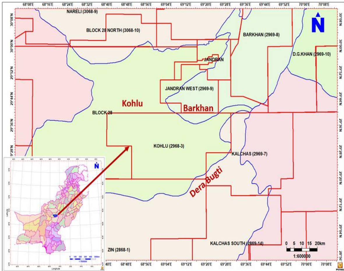
Figure-02: Districts wise location map of Kohlu Block.
