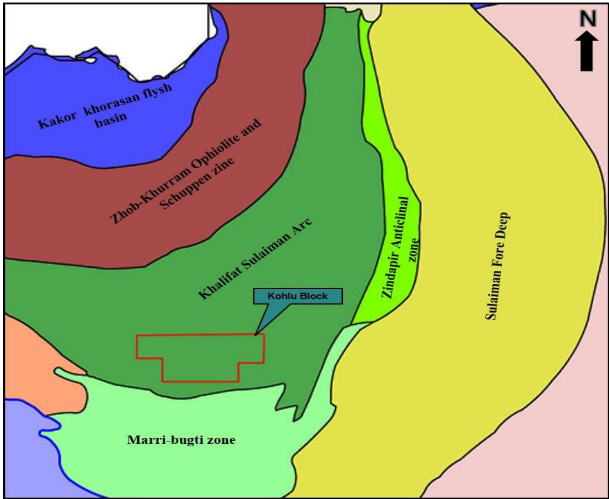
Figure-04: Tectonics of the Kohlu region.
