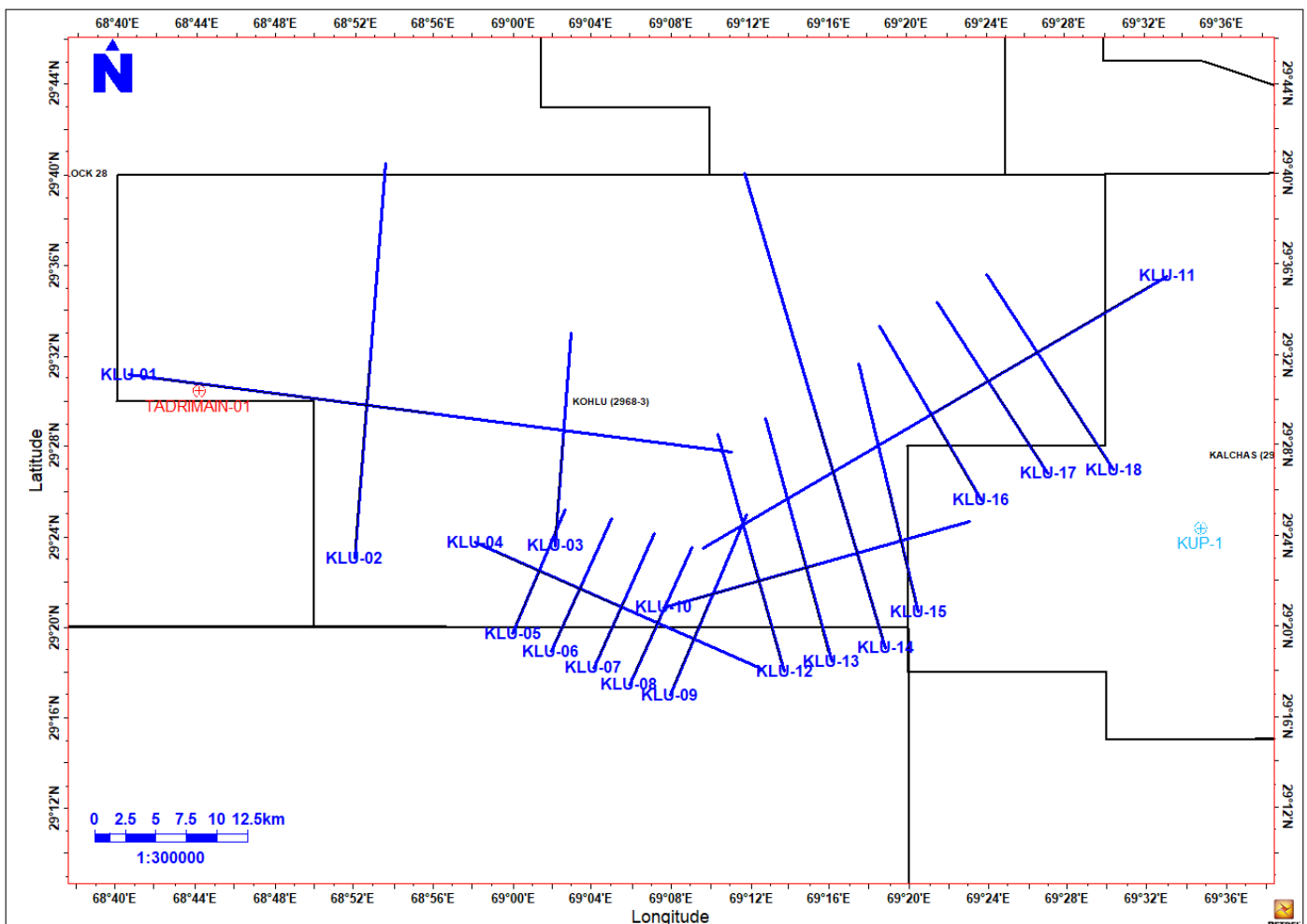
Figure-06: 2D Seismic plan of Kohlu block.
