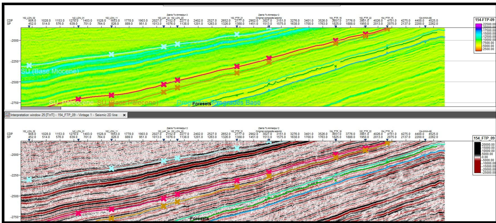
Fig.3: Inverted and Original Seismic (with horizon).
