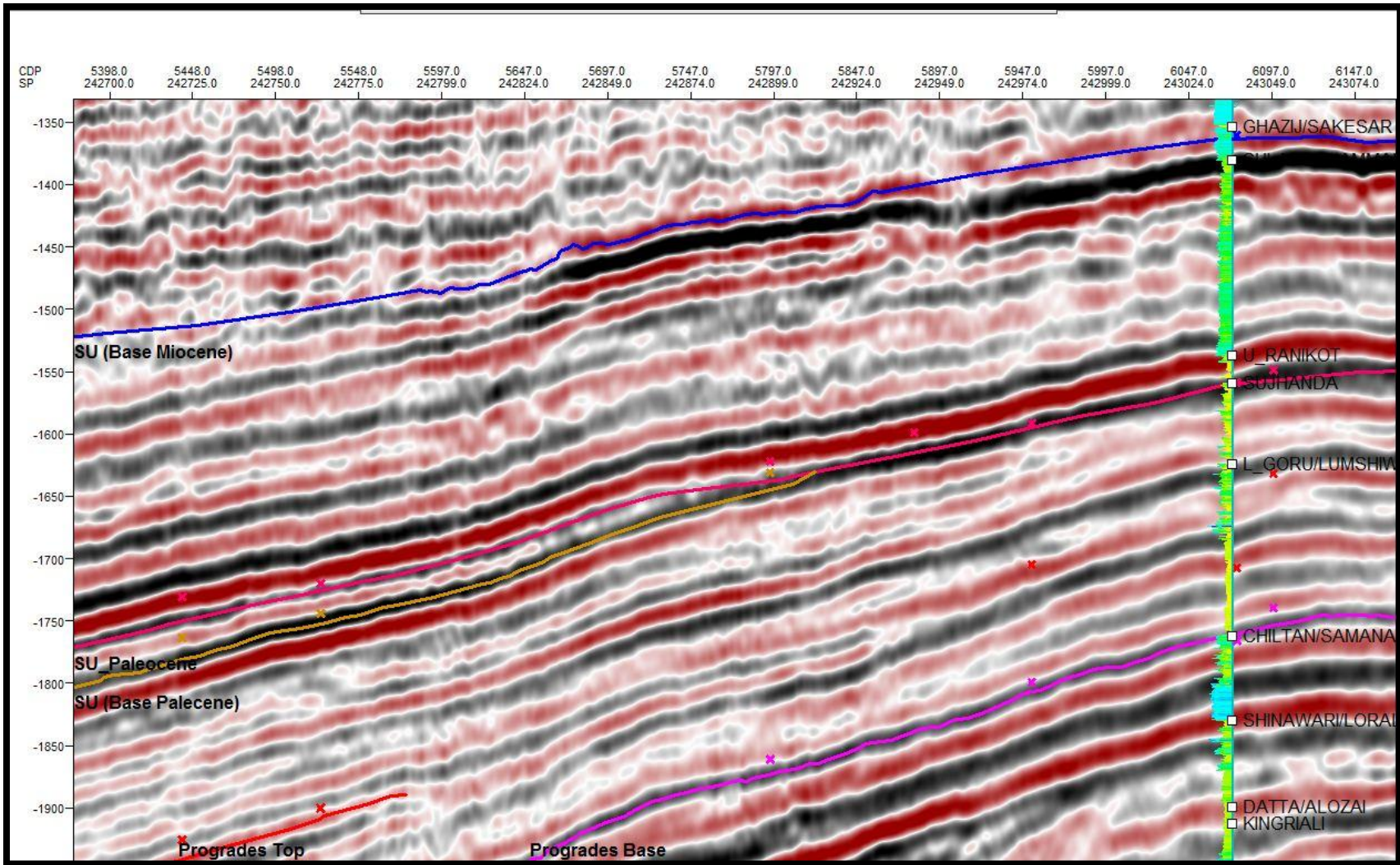
Fig.2: Seismic to Well tie (P-Impedance Log).
