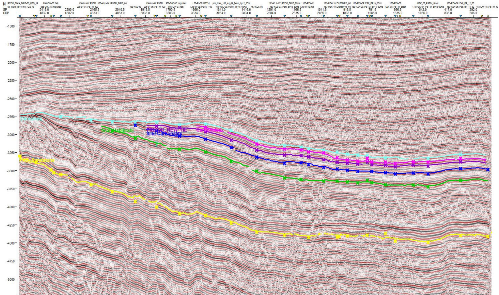
Fig.4: Seismic Strike Line Showing Stratigraphic Truncations against Base Miocene Unconformity.
