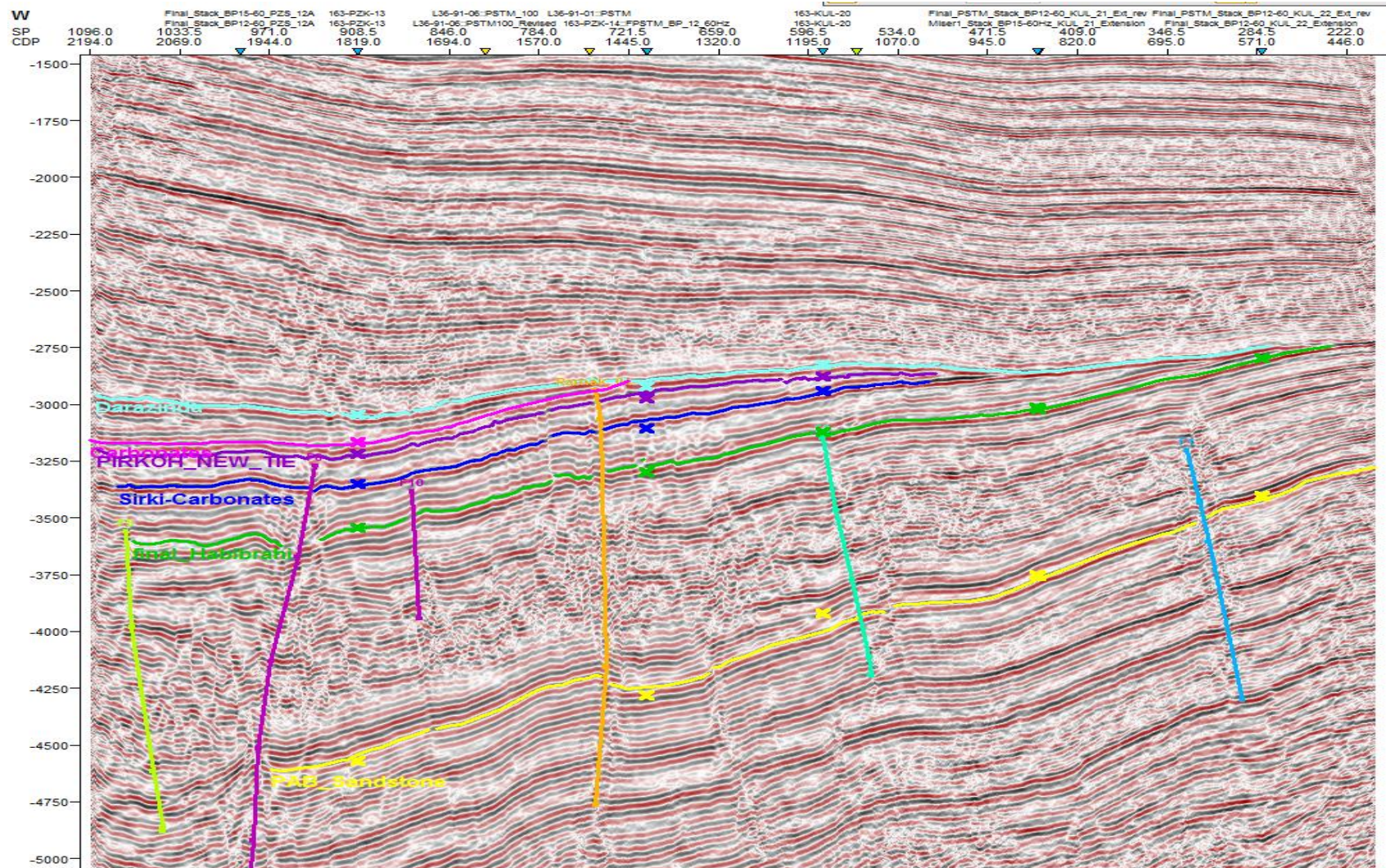
Fig.3: Seismic Dip line showing stratigraphic truncations against Base Miocene Unconformity.
