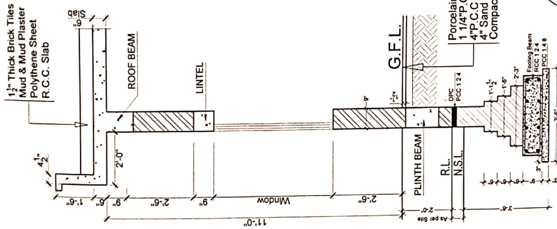
WALL & FOOTING SEC.
