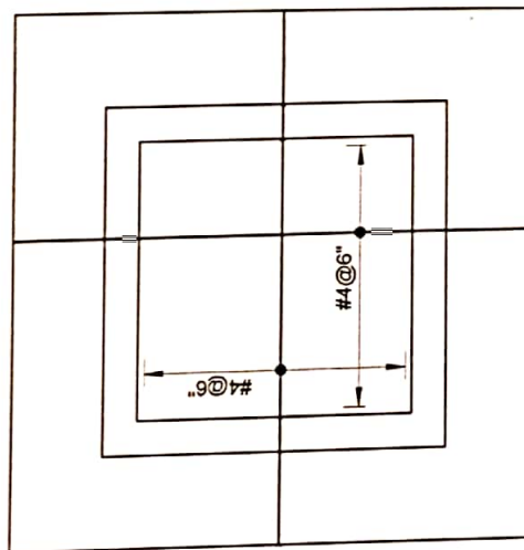
SLAB REINF. PLAN WATCH TOWER
